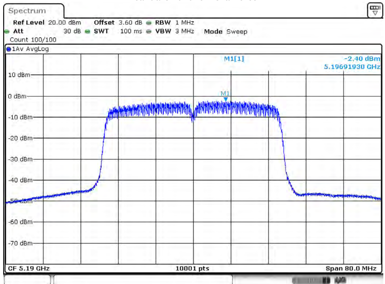
Peak transmit Power - Channel 38
