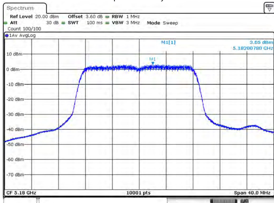
Peak Power Spectral Density – Channel 36
