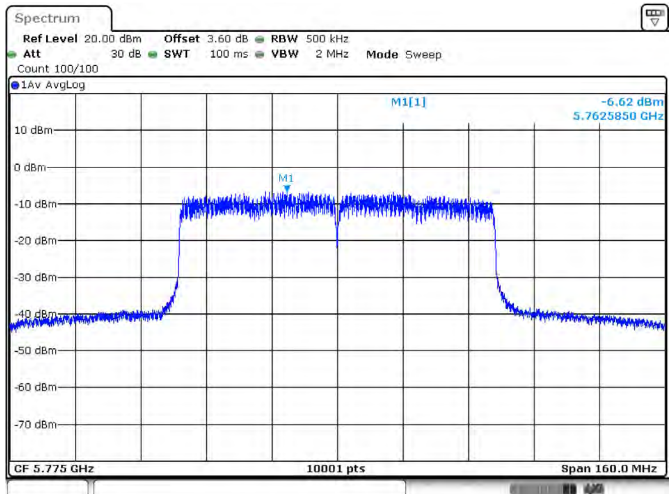
Peak transmit Power - Channel 155
