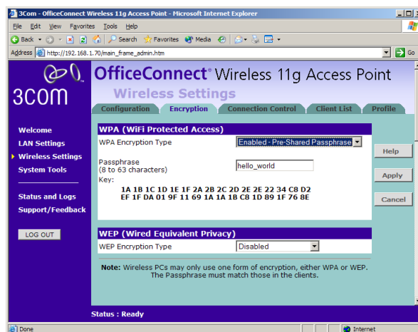
Figure 27 Encryption Keys Screen showing WPA configuration
