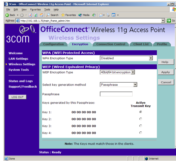
Figure 28 Encryption Keys Screen showing WEP configuration
