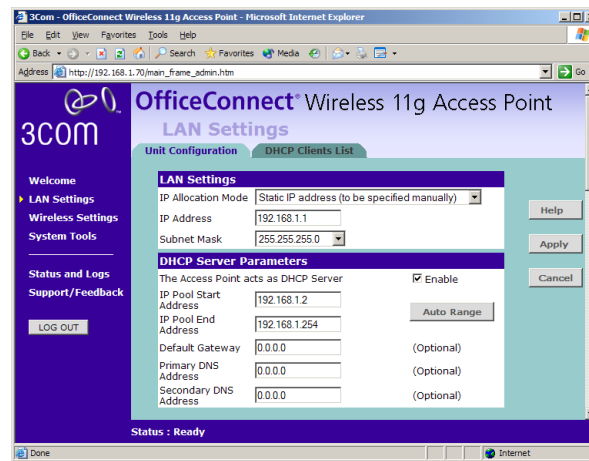
Figure 24 DHCP Server Configuration Screen
