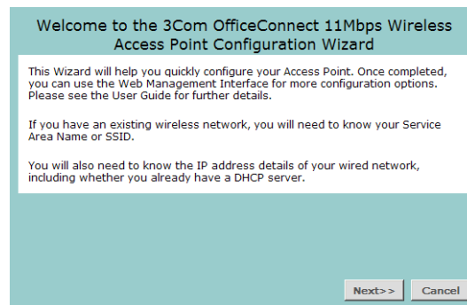
Figure 11 Wizard Screen
