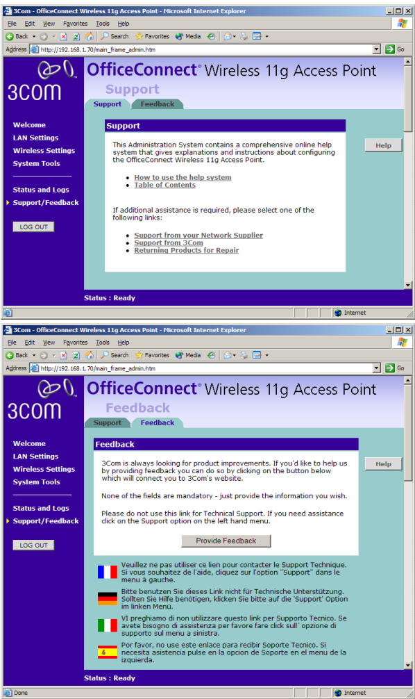
Figure 38 Support Screen
