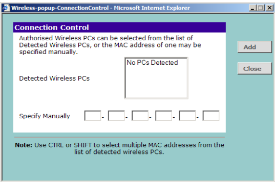
Figure 30 Connection Control Detail Screen
