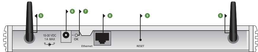
Figure 3 Access Point - Rear Panel
