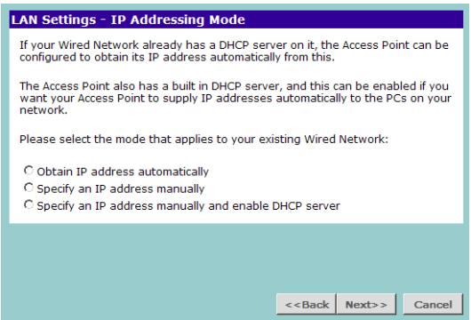
LAN Settings Figure 13 LAN Settings Screen
