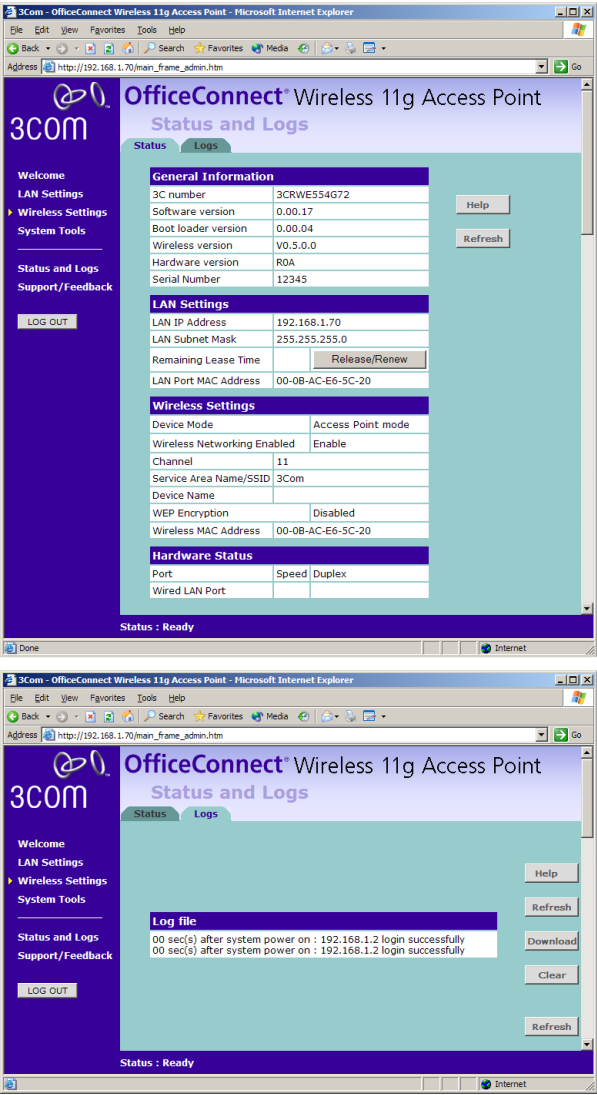
Figure 37 Status and Logs Screen
