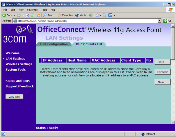
DHCP Clients List Figure 25 DHCP Clients List Screen
