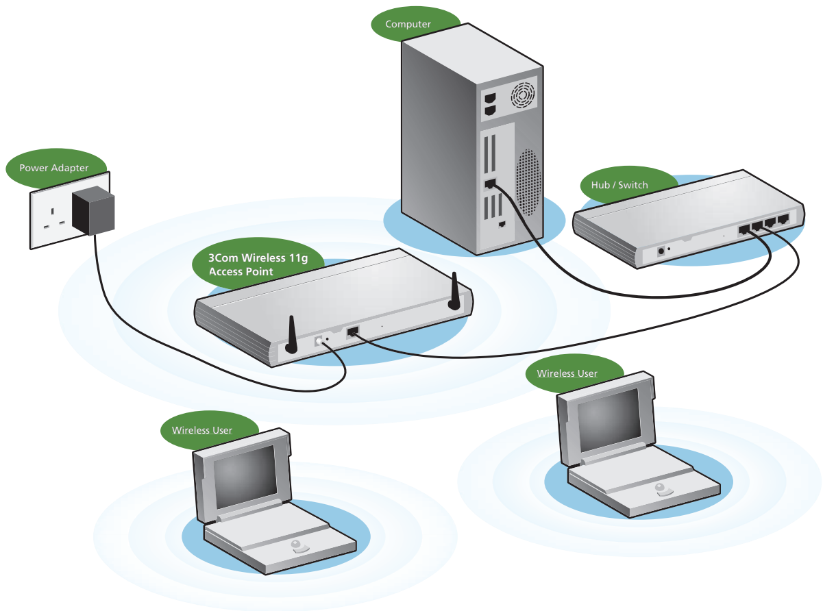
Figure 1 Example Network
