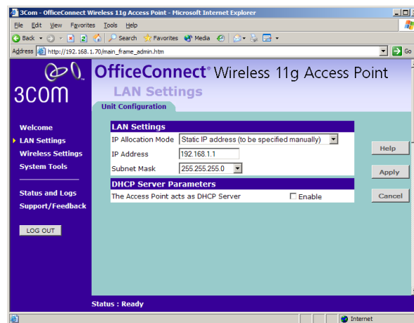
Figure 23 Unit Configuration Screen For Static IP Address
