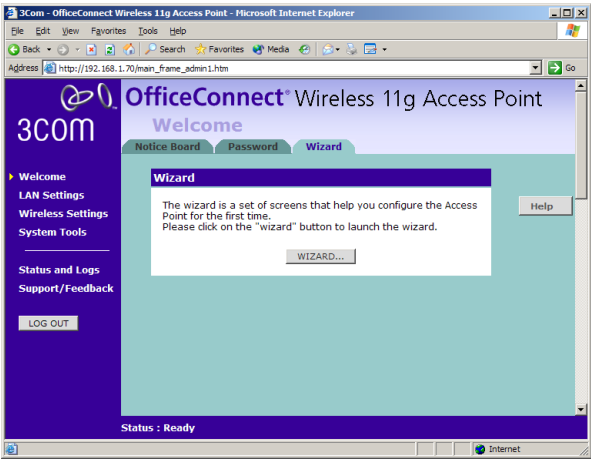
Wizard Figure 21 Wizard Screen
