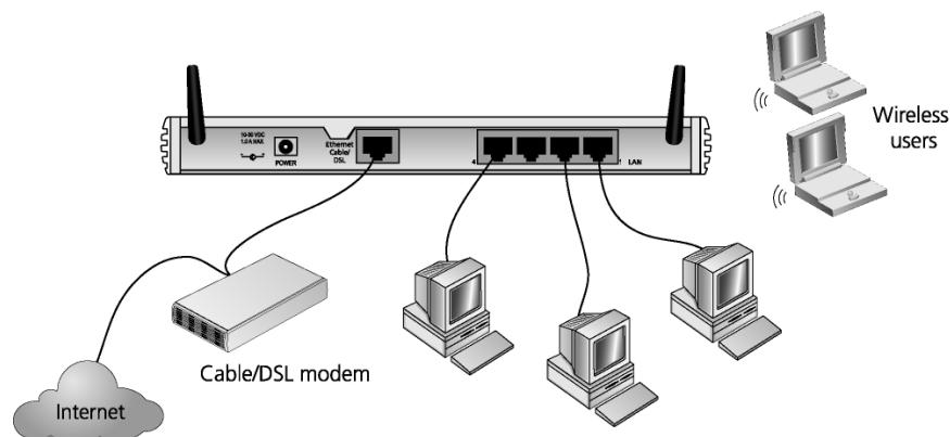
Figure 5 Connecting the Gateway
