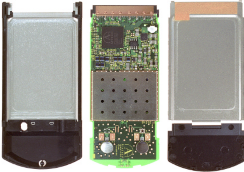
Internal Assembly View
