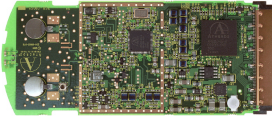
Top View of Board without shield
