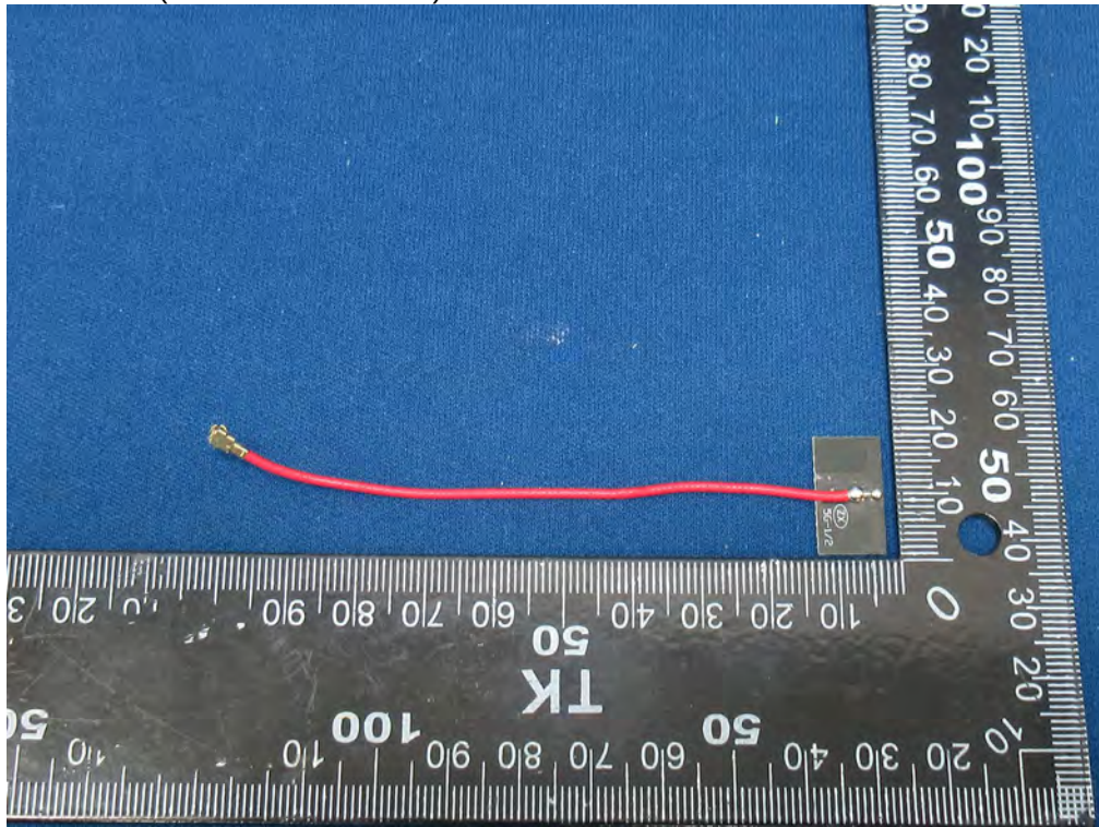
(6) EUT Photo (Wi-Fi 5 GHz – Ant. 2)
