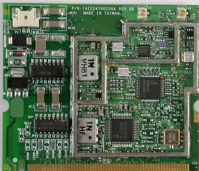
Accton WN3601A 910322R02
