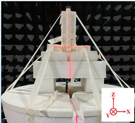
Antenna test diagram
