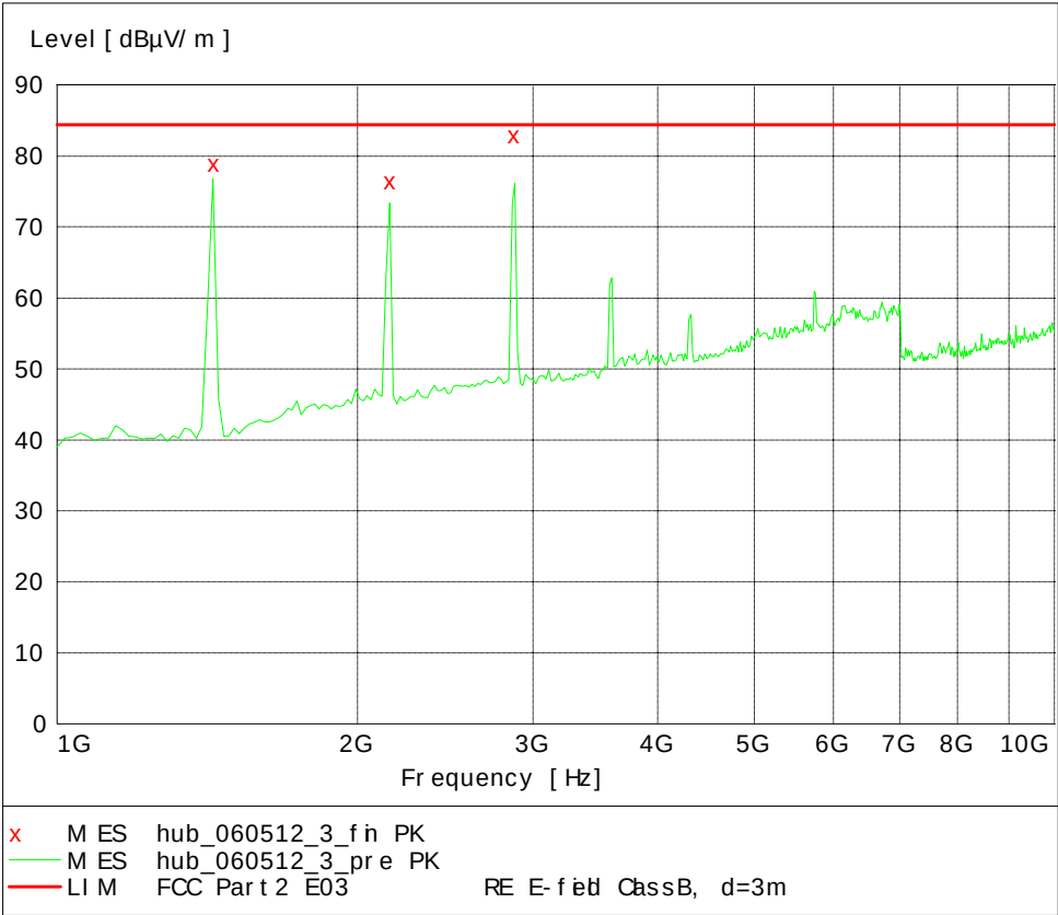
Figure 5-7: Radiated emission, 1 GHz - 10 GHz
