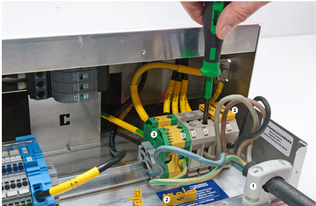
Fig. 3-13: Connecting the Power Input Cable
