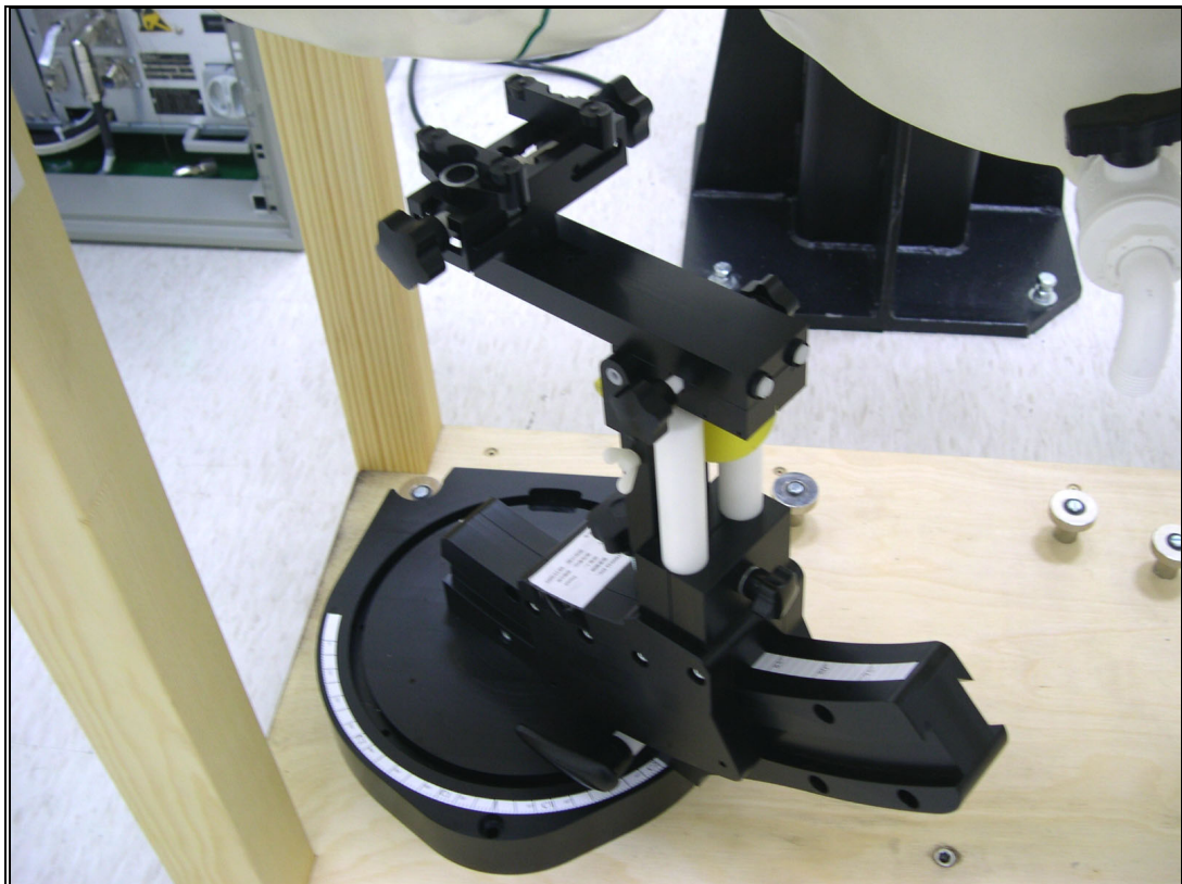
Fig. 5.5 Device Holder
