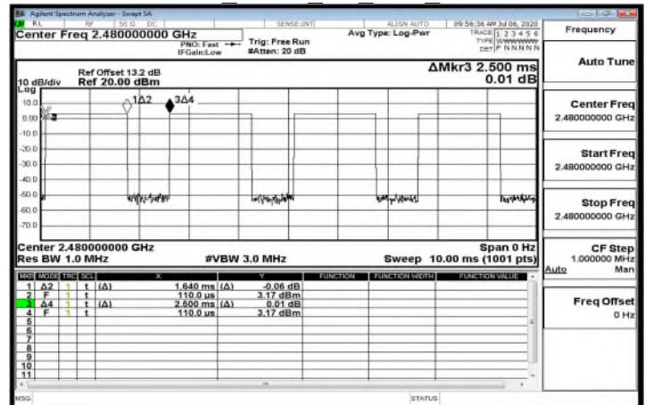
Dwell Time GFSK 1M DH3 2480MHz
