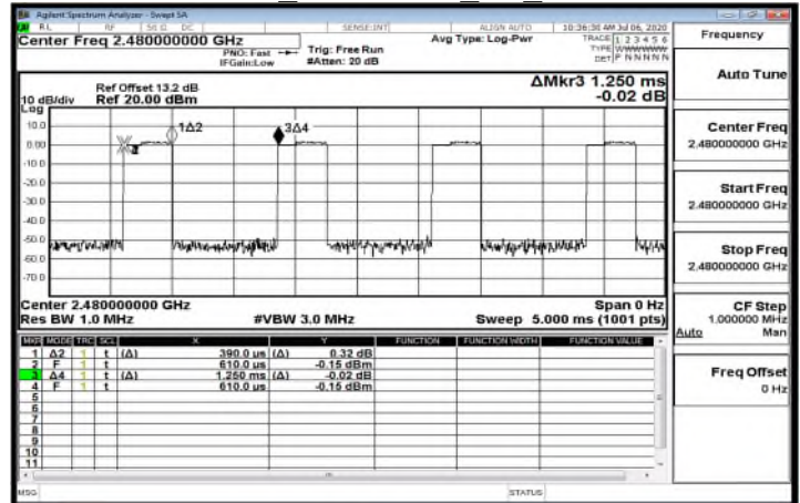
Dwell Time \pi/4 DQPSK 2M 2480MHz
