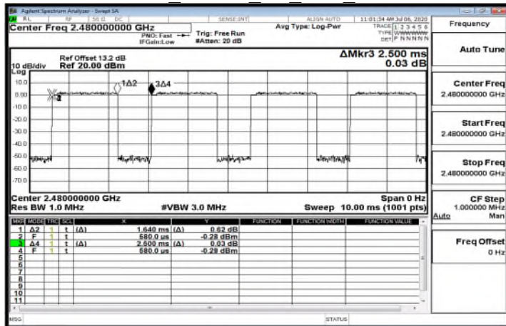
Dwell Time 8DPSK 3M DH3 2480MHz
