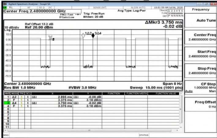
Dwell Time GFSK 1M DH5 2480MHz
