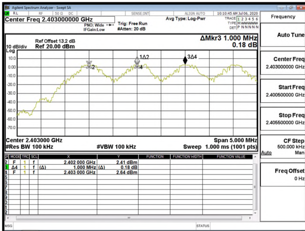
8DPSK_3M_DH5_CH0CH1CH2
