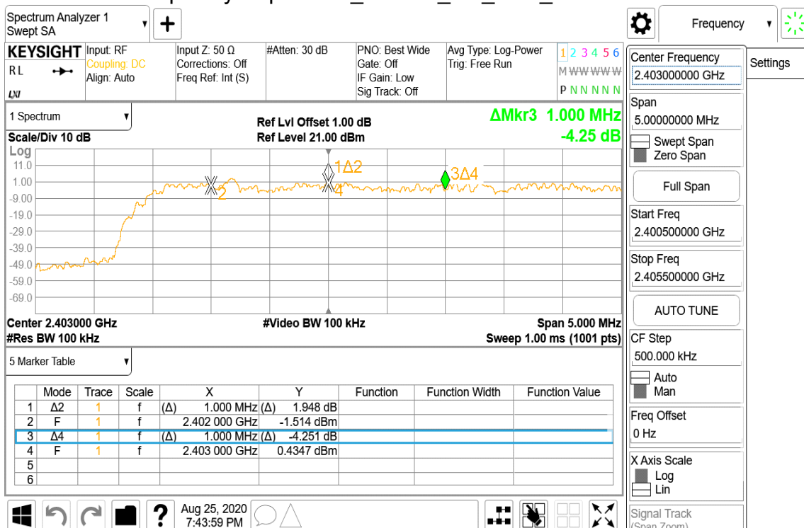
Frequency Separation 8DPSK 3M DH5 CH0CH1CH2
