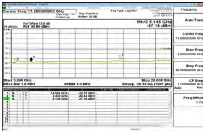
3GHz~20GHz_Band4_10MHz_QPSK_1_0_LowCH20000-1715
