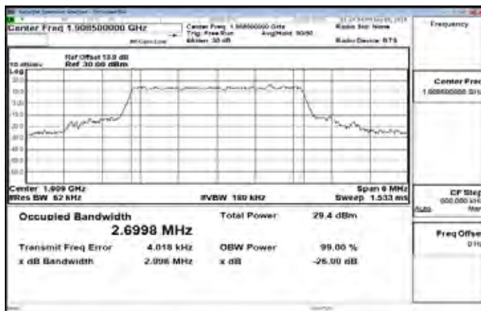
Band2_3MHz_16QAM_15_0_HighCH19185-1908.5
