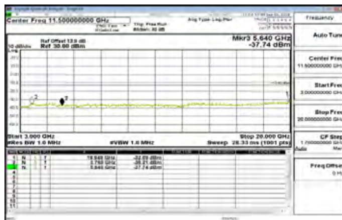
3GHz~20GHz_Band2_15MHz_QPSK_1_0_MidCH18900-1880
