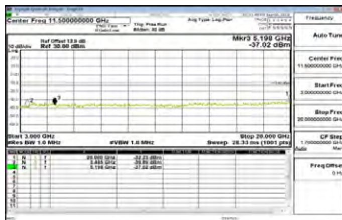
3GHz-20GHz_Band4_3MHz_QPSK_1_0_MidCH20175-1732.5
