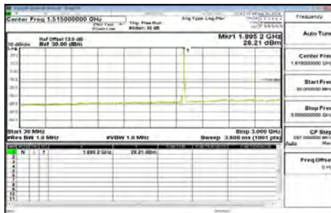
30MHz~3GHz_Band2_15MHz_QPSK_1_0_HighCH19125-1902.5
