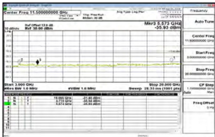
3GHz~20GHz_Band2_15MHz_QPSK_1_0_LowCH18675-1857.5
