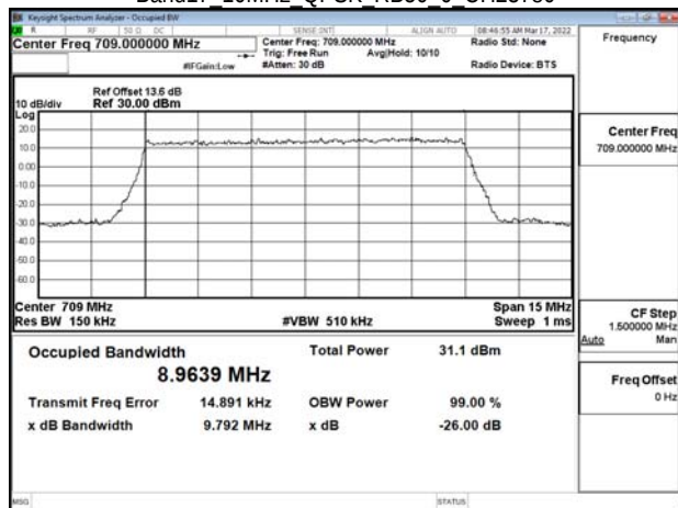
Band17 10MHz QPSK RB50_0 CH23780
