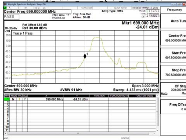
Band Edge Band12 1.4MHz QPSK RB1 5 CH23173
