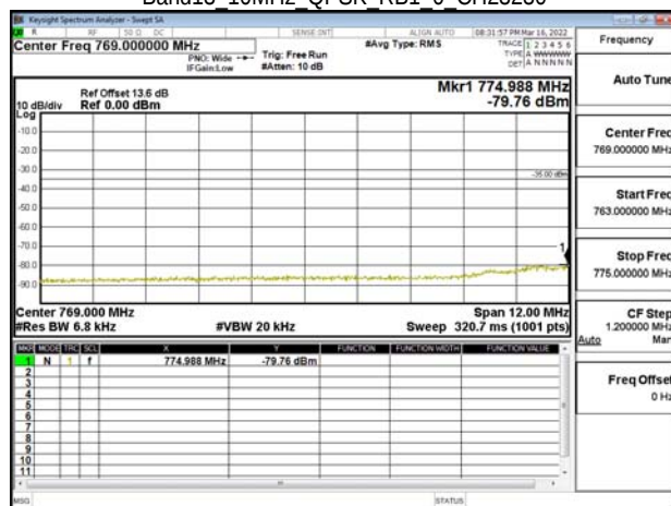
Band13 10MHz QPSK RB1 0 CH23230
