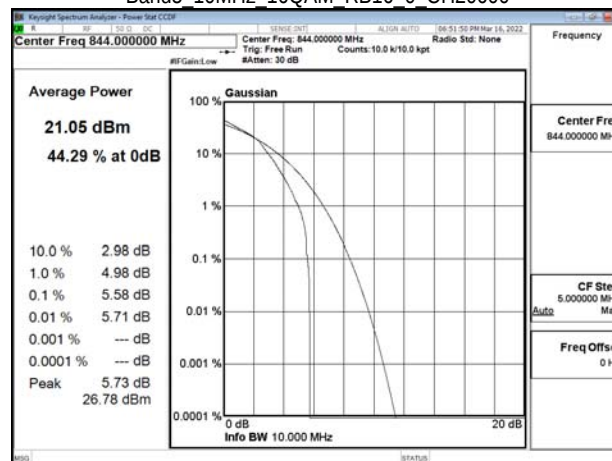
Band5 10MHz 16QAM RB16 0 CH20600
