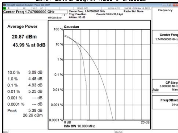
Band4 15MHz 16QAM RB16 0 CH20325
