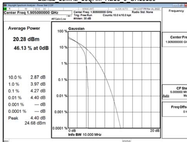
Band2 10MHz 16QAM RB16 0 CH19150
