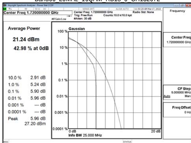
Band66 20MHz 16QAM RB18 0 CH132072
