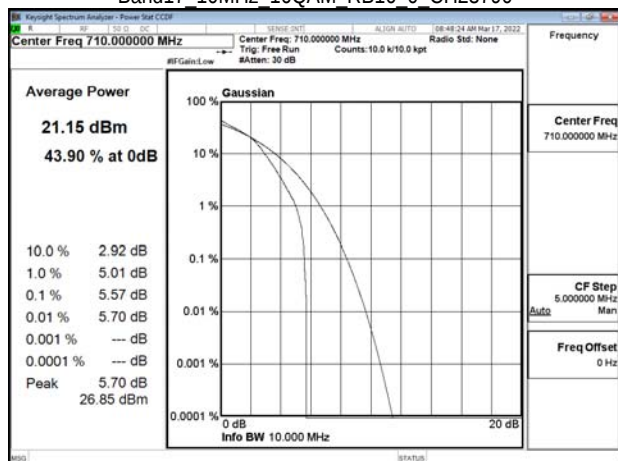
Band17 10MHz 16QAM RB16 0 CH23790
