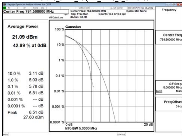
Band13 5MHz 16QAM RB25 0 CH23255
