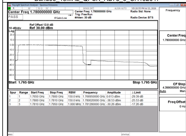
Band66 15MHz QPSK RB75 0 CH132597
