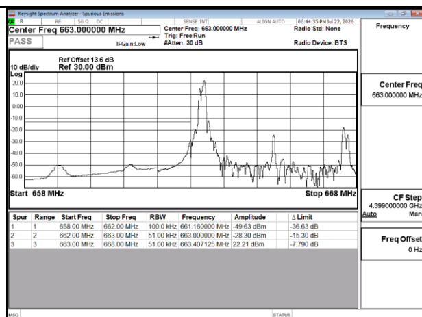
Band71 5MHz QPSK RB1 0 CH133147
