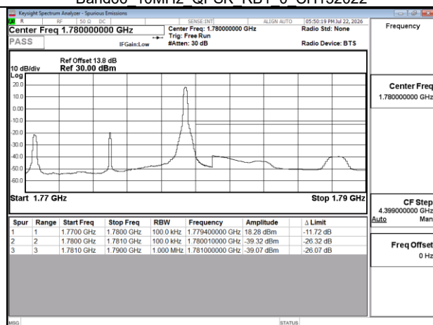
Band66 10MHz QPSK RB1 49 CH132622
