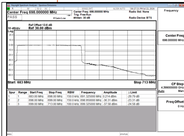
Band71 15MHz QPSK RB75 0 CH133397
