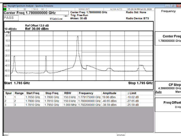
Band66 15MHz QPSK RB1 74 CH132597
