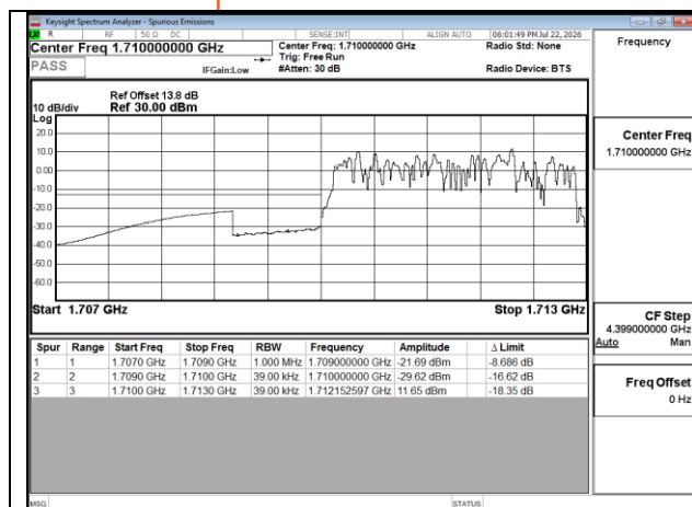
Band66 3MHz QPSK RB15 0 CH131987
