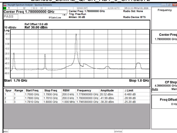
Band66 20MHz QPSK RB1 99 CH132572
