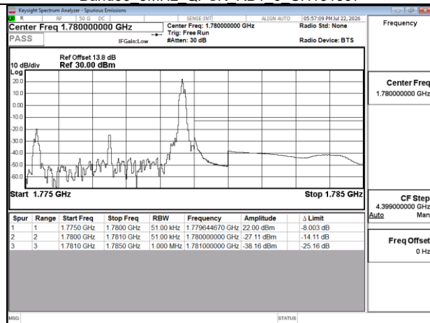
Band66 5MHz QPSK RB1 24 CH132647
