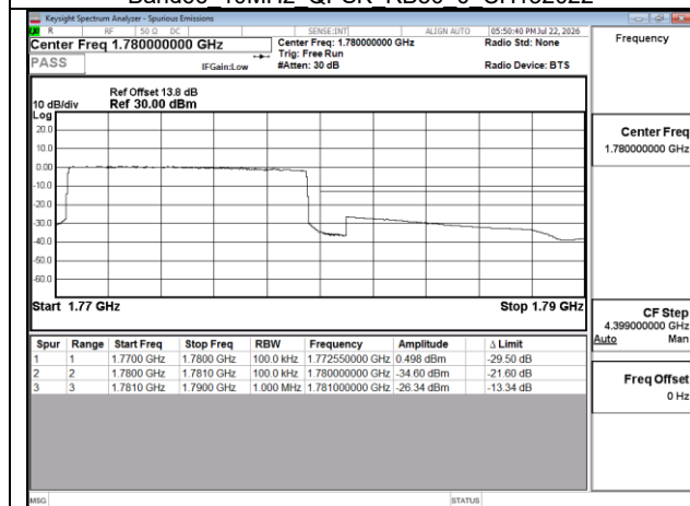
Band66 10MHz QPSK RB50 0 CH132622
