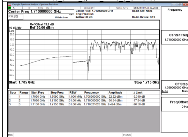
Band66 5MHz QPSK RB25 0 CH131997
