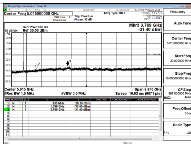
Band5 5MHz QPSK RB1 0 CH20525 below 18G
