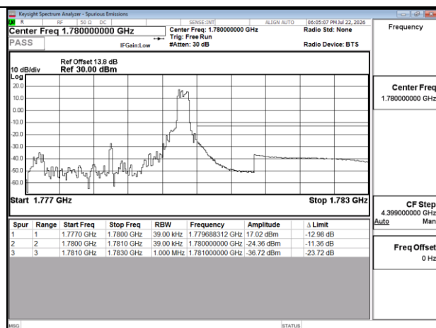
Band66 3MHz QPSK RB1 14 CH132657
