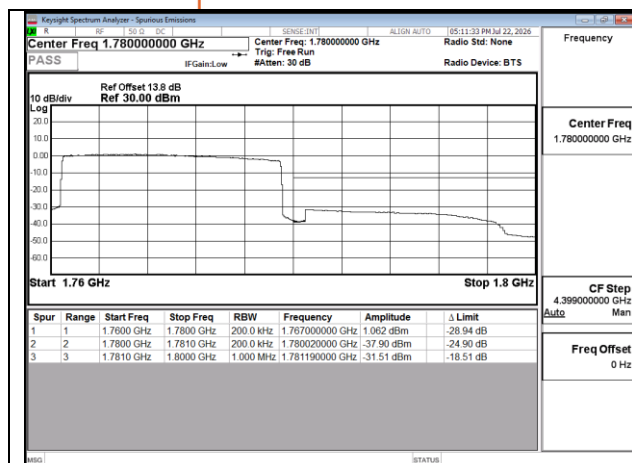
Band66 20MHz QPSK RB100 0 CH132572
