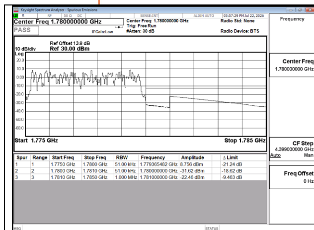
Band66 5MHz QPSK RB25 0 CH132647
