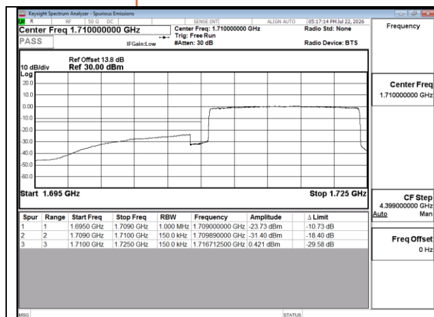
Band66 15MHz QPSK RB75 0 CH132047
