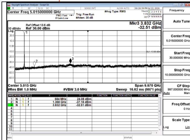
Band71 15MHz QPSK RB1 0 CH133397 below 18G
