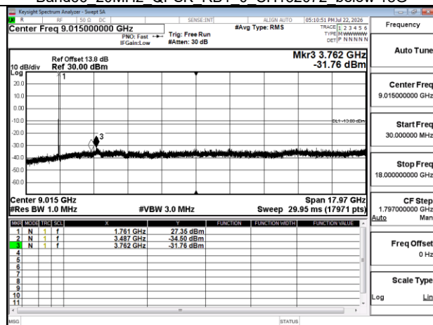
Band66 20MHz QPSK RB1 0 CH132572 below 18G
