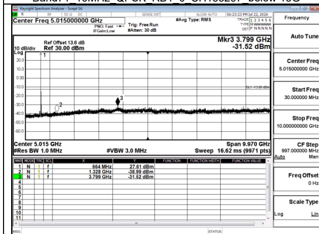
Band71 15MHz QPSK RB1 0 CH133197 below 18G
