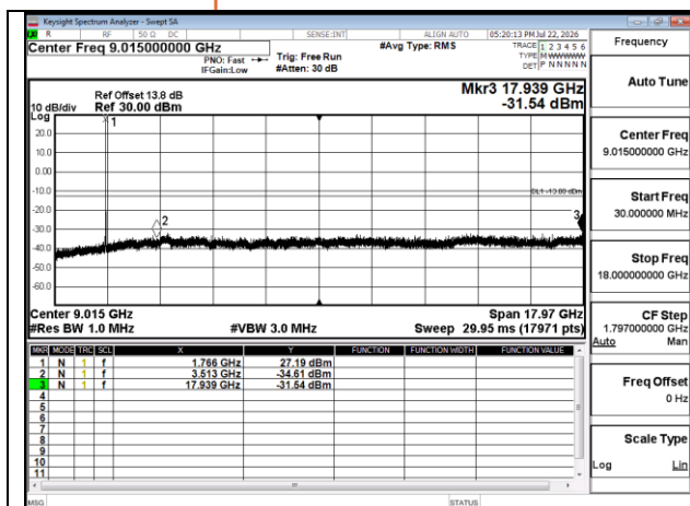
Band66 15MHz QPSK RB1 0 CH132597 below 18G
