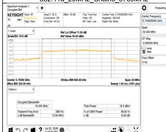
802.11a_20MHz_Chain0_5745MHz
