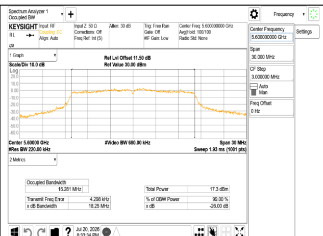
802.11a_20MHz_Chain0_5600MHz
