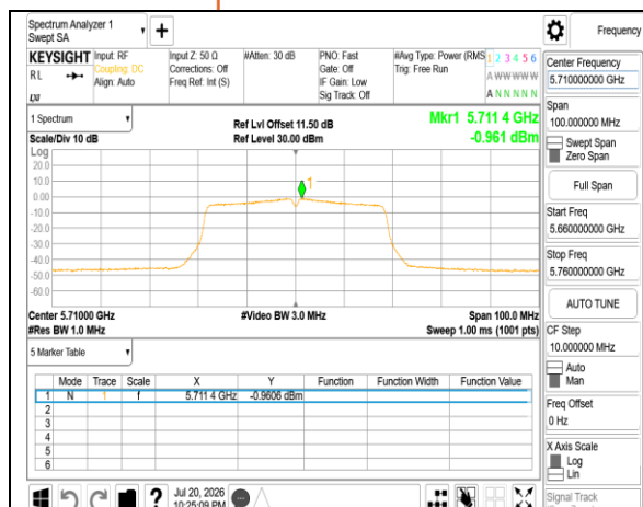
802.11n 40MHz Chain1 5710MHz UNII 2C
