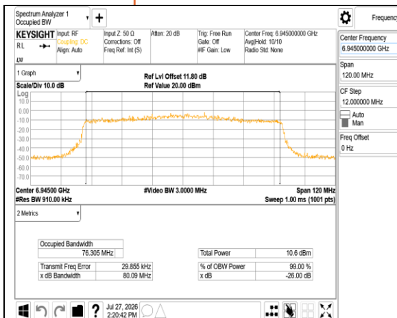
802.11ax_80MHz_Chain1_6945MHz
