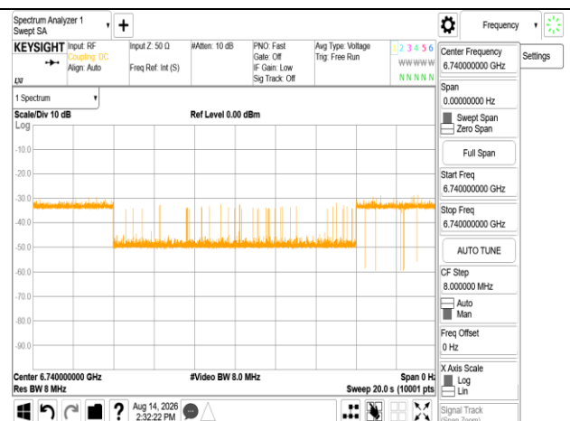
ax 160M 6665MHz Int6740MHz -67.15dBm Minimal
