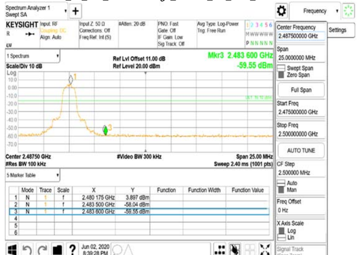
FCC_15_247_BTBand Edge_8DPSK_3M_DH5_2480MHz
