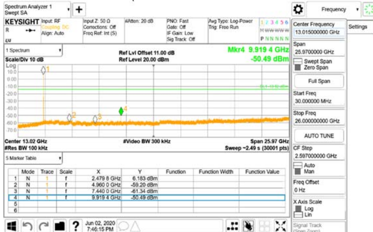
FCC_15_247_BTSpurious Emission_GFSK_1M_DH5_2480MHz
