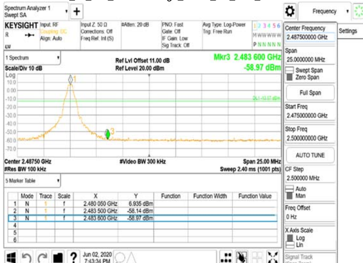
FCC_15_247_BTBand Edge_GFSK_1M_DH5_2480MHz
