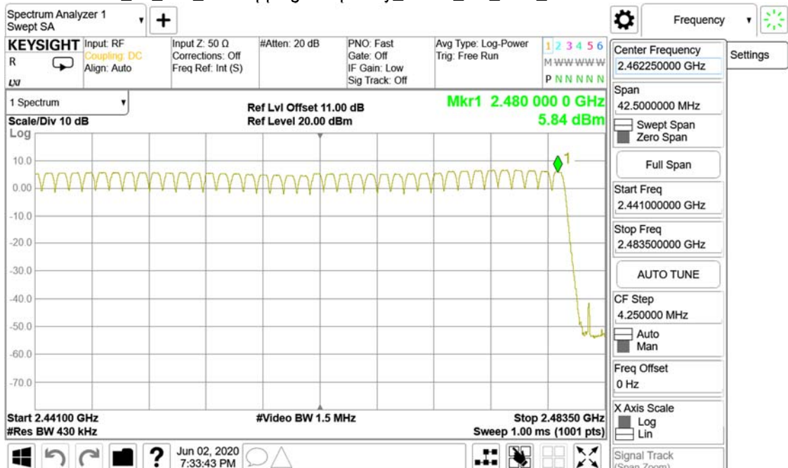
FCC_15_247_BT Hopping Frequency_GFSK_1M_DH5_2441-2480
