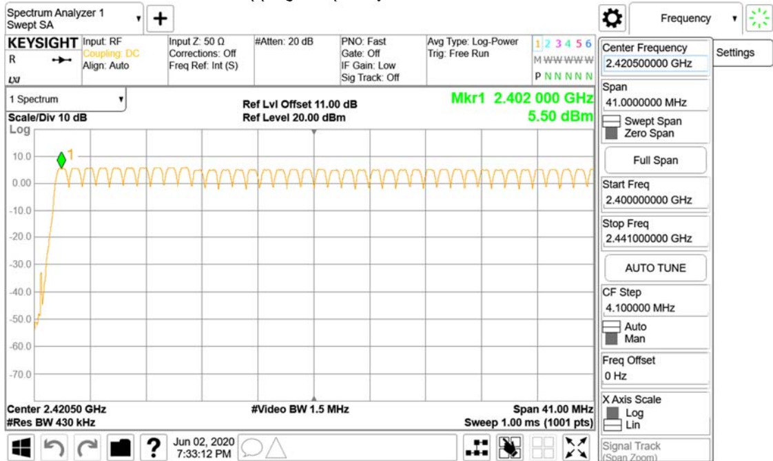
FCC_15_247_BT Hopping Frequency_GFSK_1M_DH5_2400-2441
