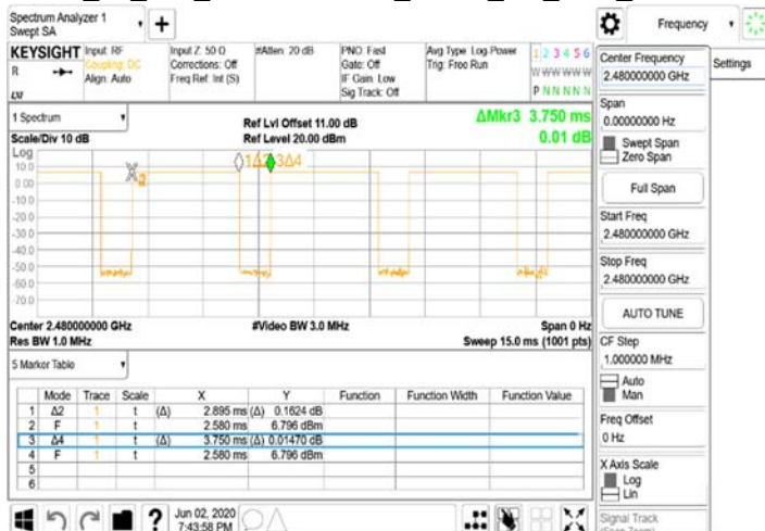
FCC_15_247_BT\Dwell Time_GFSK_1M_DH5_2480MHz
