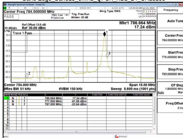
Band Edge Band13 5MHz QPSK RB25 0 CH23205
