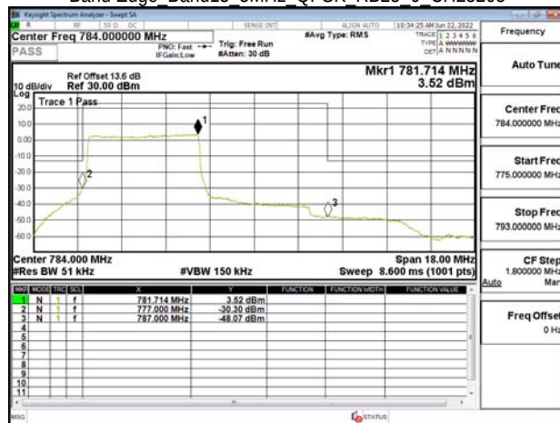
Band Edge Band13 5MHz QPSK RB25 0 CH23255
