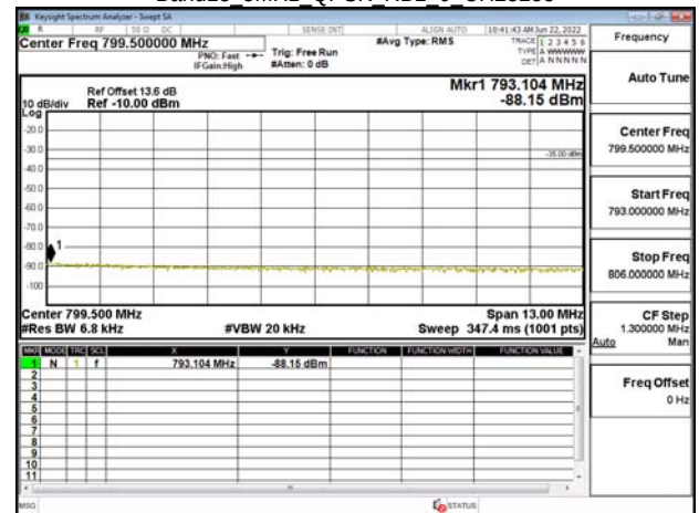
Band13 5MHz QPSK RB1 0 CH23255
