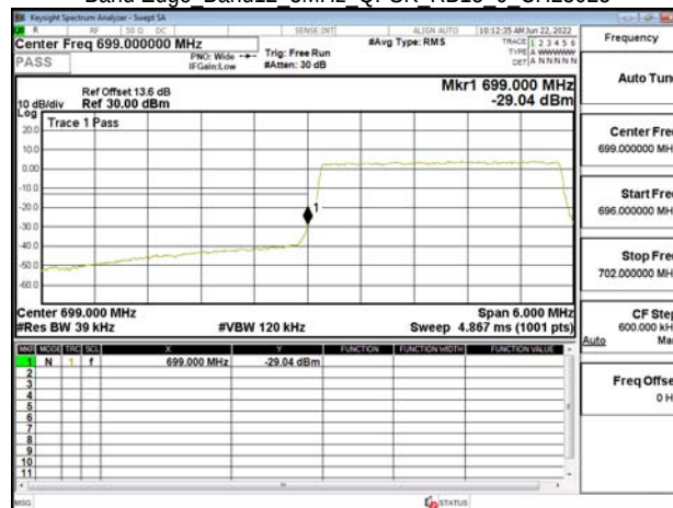
Band Edge Band12 3MHz QPSK RB15 0 CH23165
