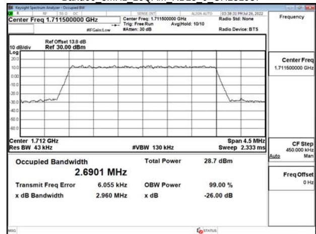
Band66 3MHz 16QAM RB15 0 CH131987
