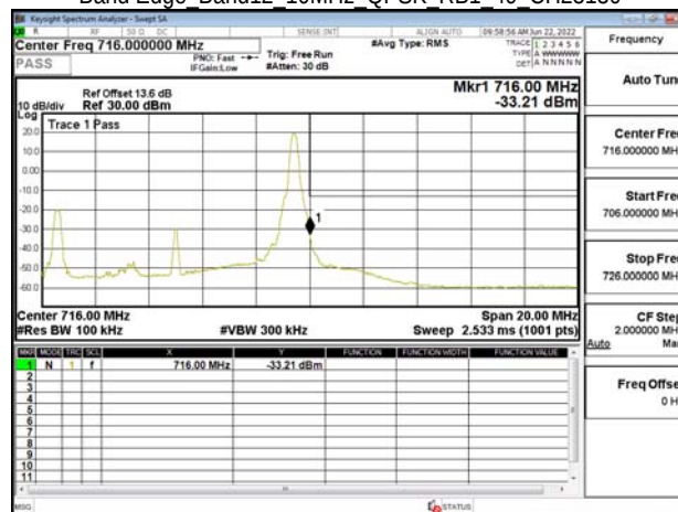
Band Edge Band12 10MHz QPSK RB1 49 CH23130
