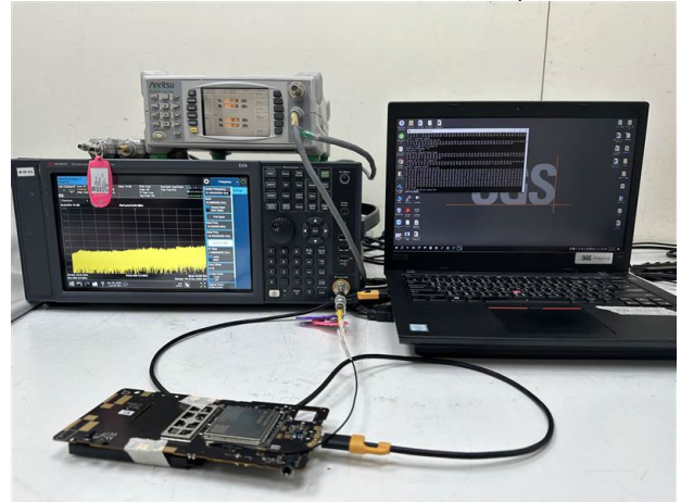
Part_15_225_NFC_Conducted_Setup
