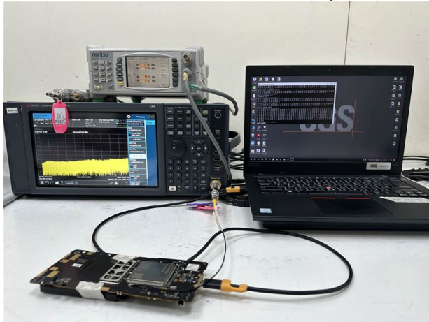
Part_15.247_WLAN_Conducted_Setup
