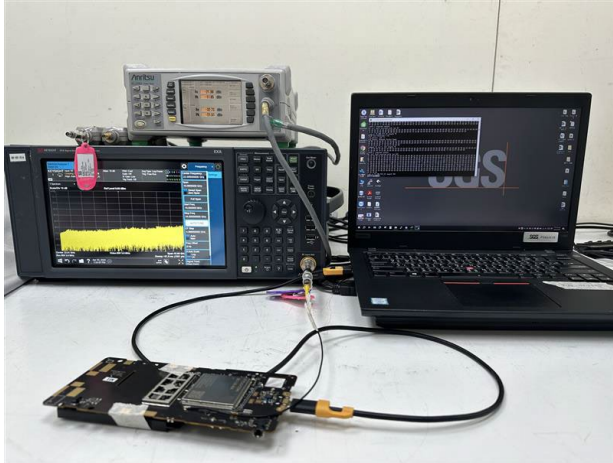
Part_15.247_WLAN_Conducted_Setup
