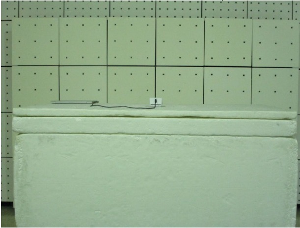
Part_15.247_BLE_Radiated_Setup
