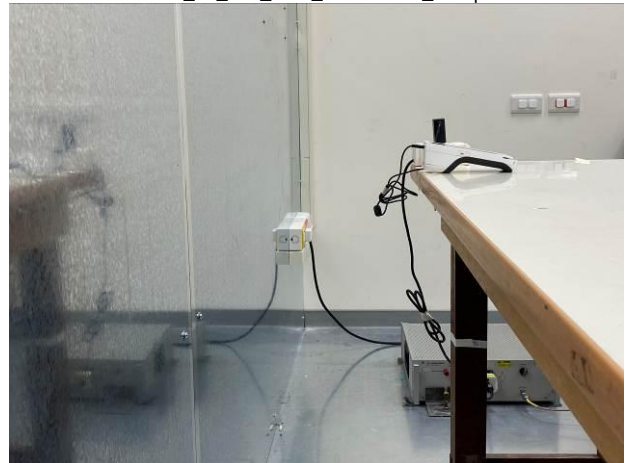
Part_15_225_NFC_Conduction_Setup
