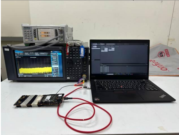
Part_15.247_WLAN 2.4GHz_Conducted_Setup
