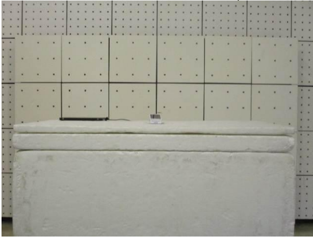
Part_22_24_27_LTE_Radiated_Setup
