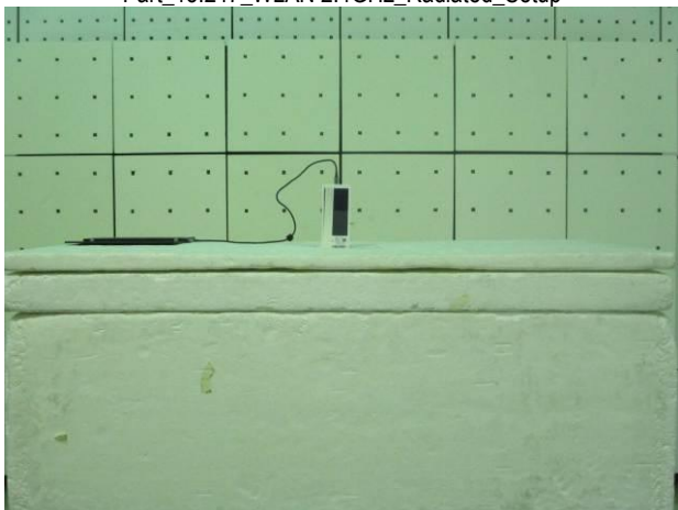
Part_15.247_WLAN 2.4GHz_Radiated_Setup
