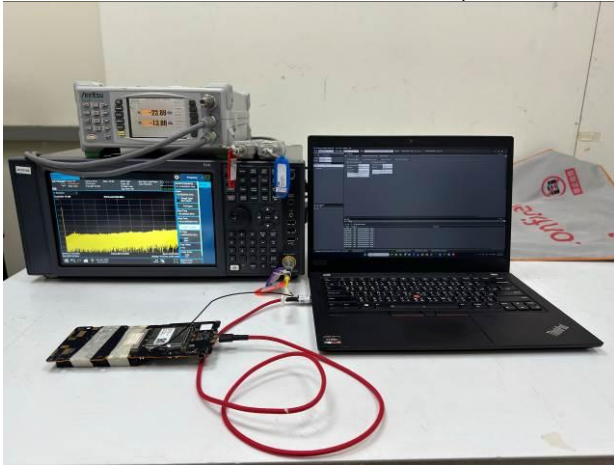
Part_15.247_BT_Conducted_Setup
