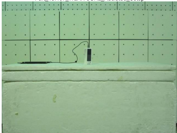
Part_15.407_WLAN 5GHz_Radiated_Setup
