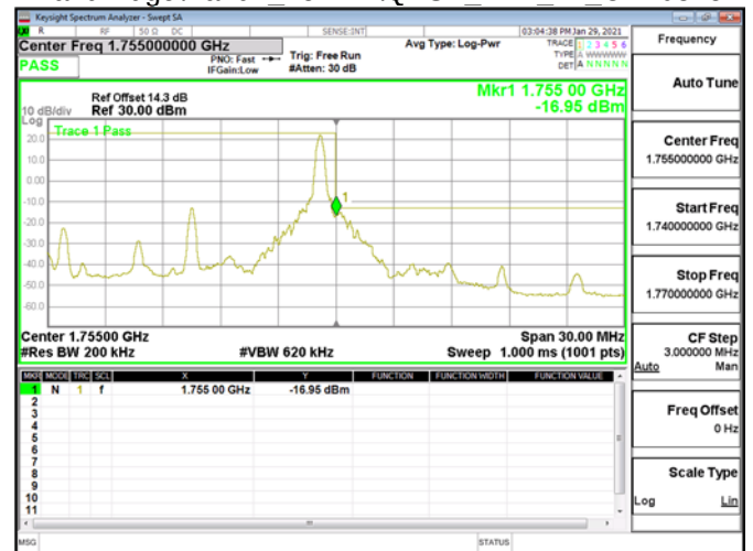
Band Edge\Band4 15MHz\QPSK RB1 74 CH20325
