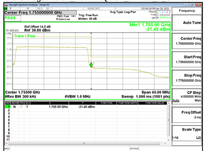
Band Edge\Band4 20MHz\QPSK RB100 0 CH20300
