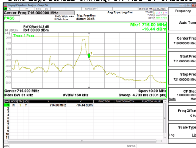
Band Edge\Band12 5MHz\QPSK RB1 24 CH23155
