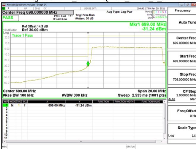
Band Edge\Band12 10MHz\QPSK RB50 0 CH23060
