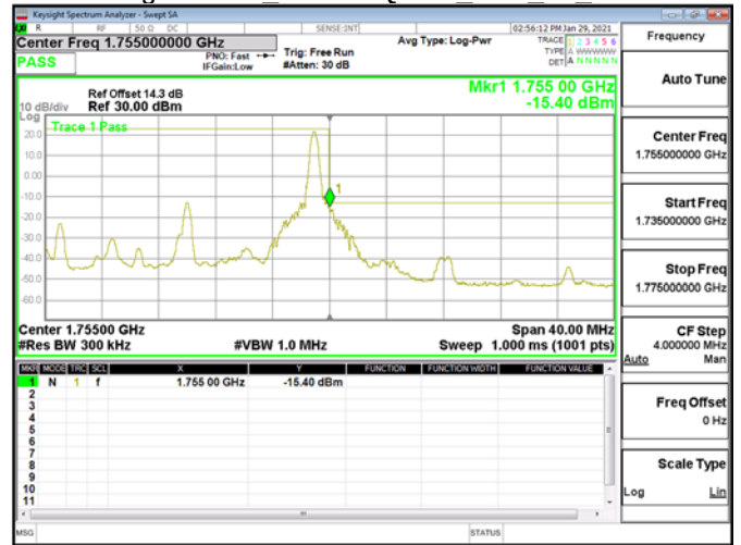
Band Edge\Band4 20MHz\QPSK RB1 99 CH20300
