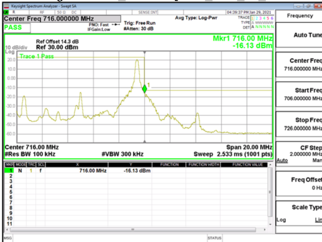
Band Edge\Band12 10MHz\QPSK RB1 49 CH23130
