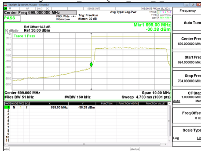
Band Edge\Band12 5MHz\QPSK RB25 0 CH23035
