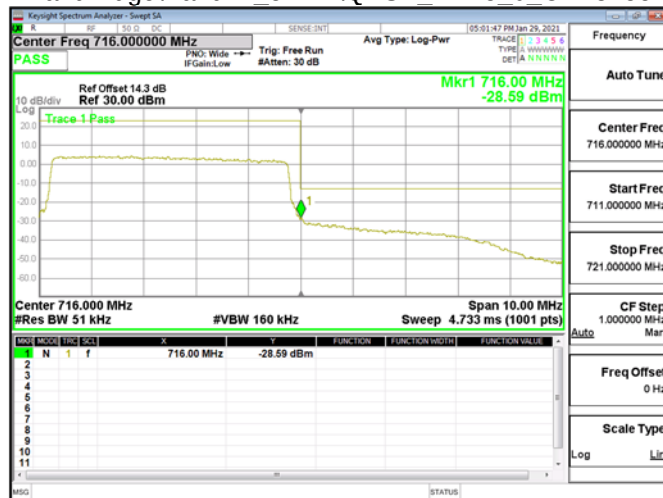
Band Edge\Band12 5MHz\QPSK RB25 0 CH23155
