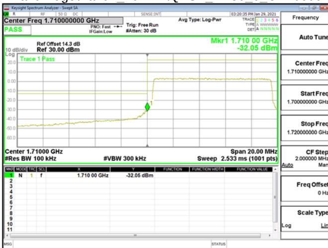
Band Edge\Band4 10MHz\QPSK RB50 0 CH20000
