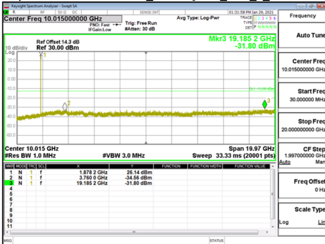
Spurious Emission\Band2 5MHz\QPSK RB1 0 CH18900
