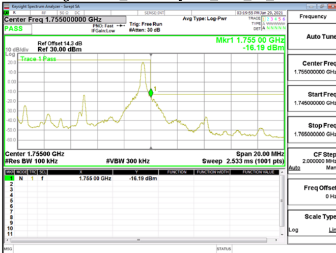
Band Edge\Band4 10MHz\QPSK RB1 49 CH20350
