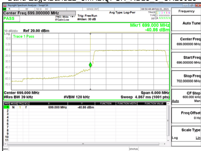
Band Edge\Band12 3MHz\QPSK RB15 0 CH23025
