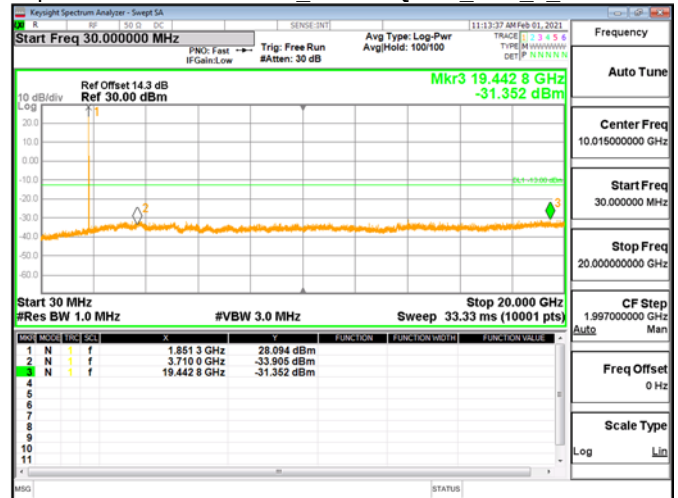
Spurious Emission\Band2 10MHz\QPSK RB1 0 CH18650
