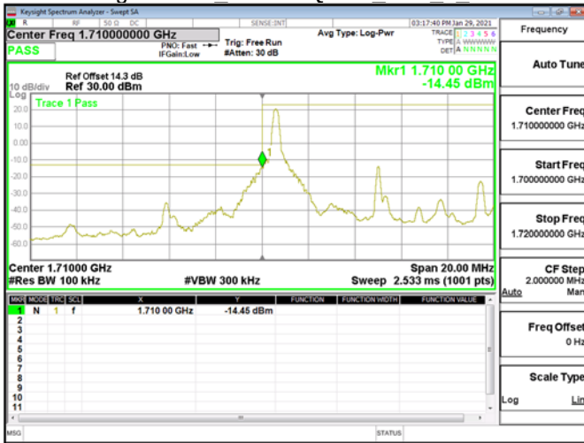
Band Edge\Band4 10MHz\QPSK RB1 0 CH20000
