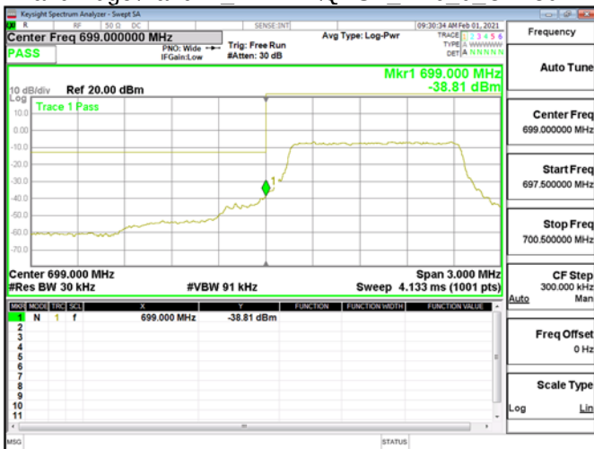
Band Edge\Band12_1.4MHz\QPSK_RB6_0_CH23017
