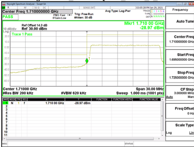
Band Edge\Band4 15MHz\QPSK RB75 0 CH20025
