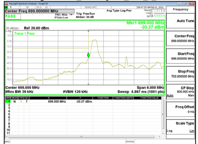
Band Edge\Band12_3MHz\QPSK_RB1_0_CH23025
