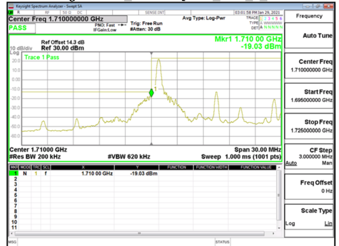
Band Edge\Band4 15MHz\QPSK RB1 0 CH20025
