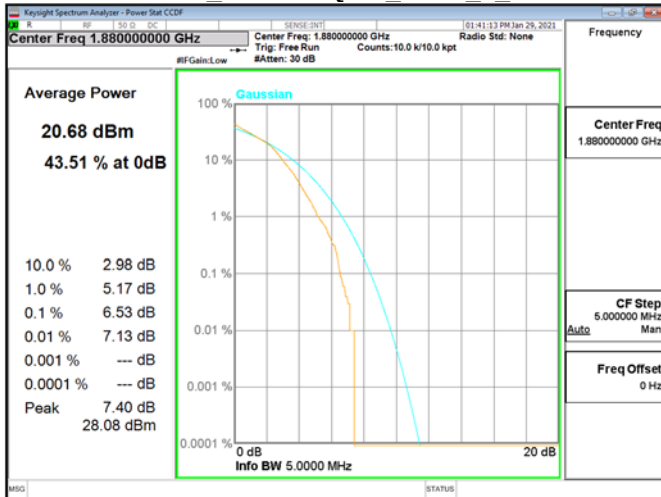
CCDF\Band2 5MHz\16QAM RB25 0 CH18900
