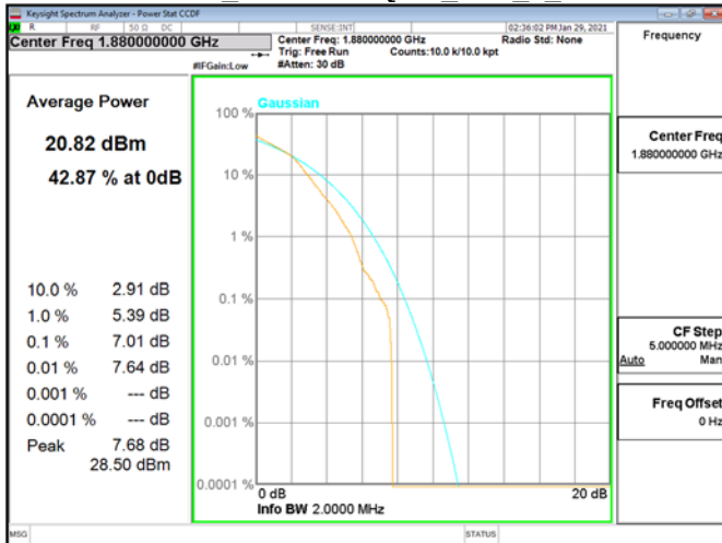
CCDF\Band2 1.4MHz\16QAM RB6 0 CH18900
