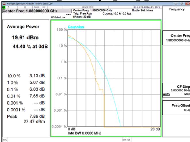
CCDF\Band2 15MHz\16QAM RB75 0 CH18900
