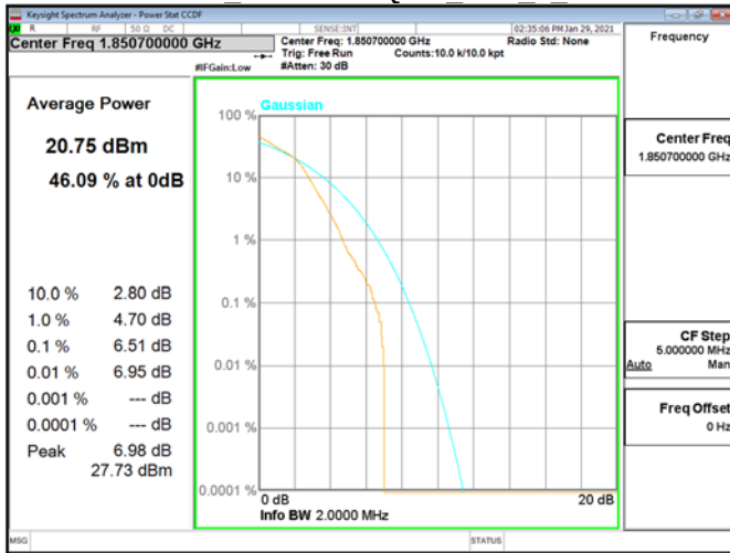
CCDF\Band2 1.4MHz\16QAM RB6 0 CH18607
