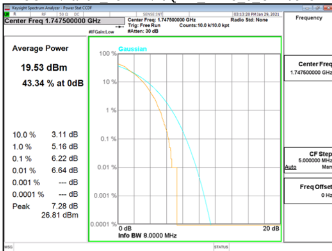
CCDF\Band4 15MHz\16QAM RB75 0 CH20325
