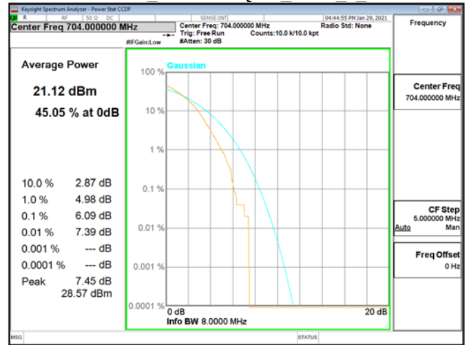
CCDF\Band12 10MHz\16QAM RB50 0 CH23060
