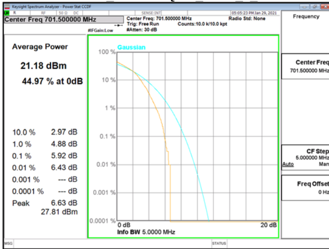
CCDF\Band12 5MHz\16QAM RB25 0 CH23035
