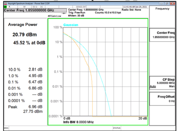
CCDF\Band2 10MHz\16QAM RB50 0 CH18650
