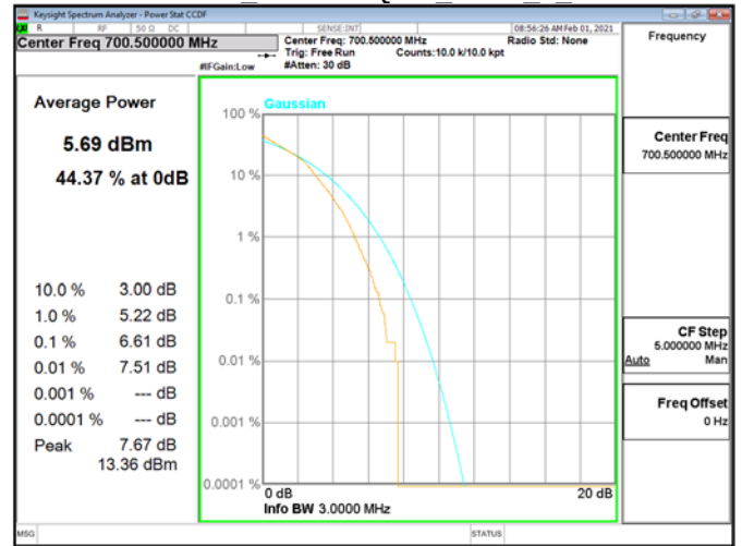
CCDF\Band12 3MHz\16QAM RB15 0 CH23025
