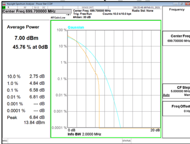
CCDF\Band12 1.4MHz\16QAM RB6 0 CH23017
