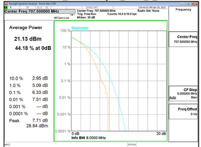
CCDF\Band12 10MHz\16QAM RB50 0 CH23095
