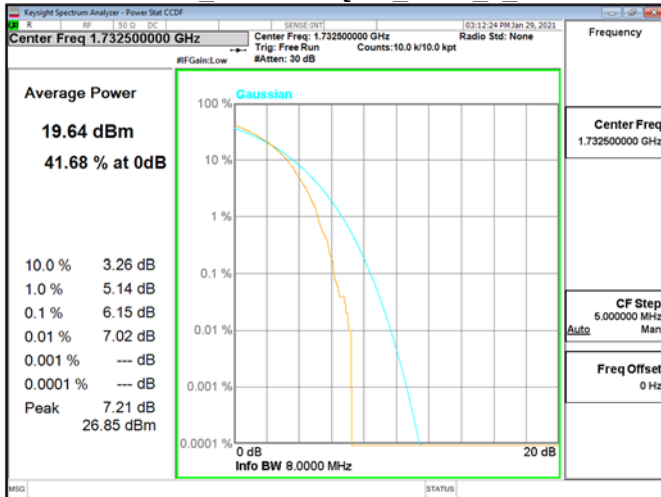
CCDF\Band4 15MHz\16QAM RB75 0 CH20175
