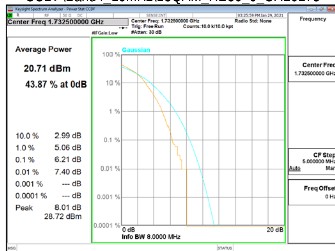
CCDF\Band4 10MHz\16QAM RB50 0 CH20175
