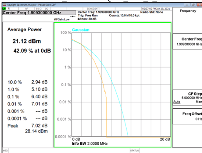
CCDF\Band2 1.4MHz\16QAM RB6 0 CH19193
