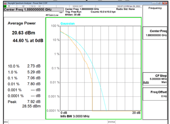
CCDF\Band2 3MHz\16QAM RB15 0 CH18900
