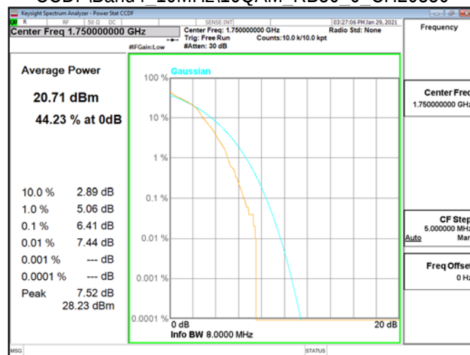
CCDF\Band4 10MHz\16QAM RB50 0 CH20350
