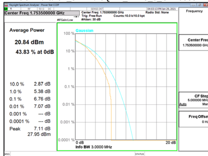
CCDF\Band4 3MHz\16QAM RB15 0 CH20385
