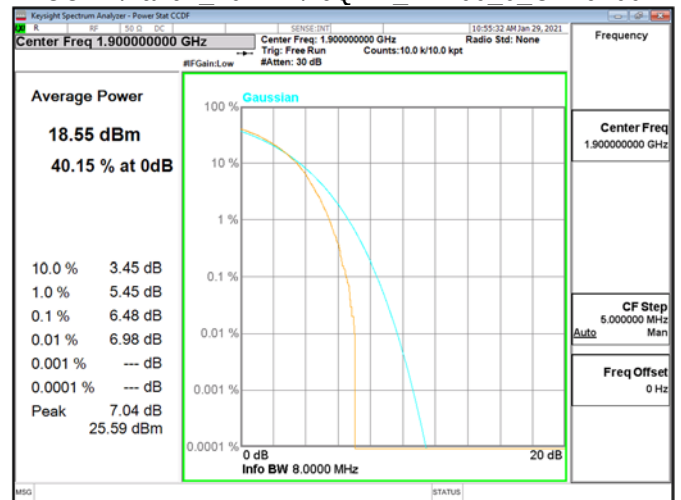
CCDF\Band2 20MHz\16QAM RB100 0 CH19100
