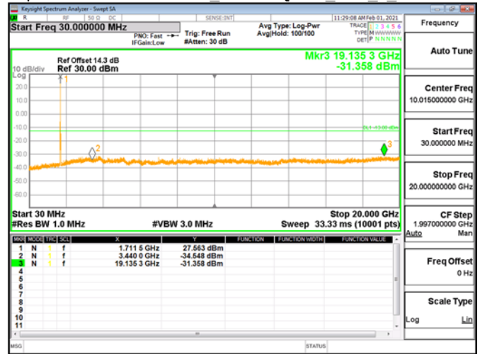
Spurious Emission\Band4 20MHz\QPSK RB1_0_CH20050
