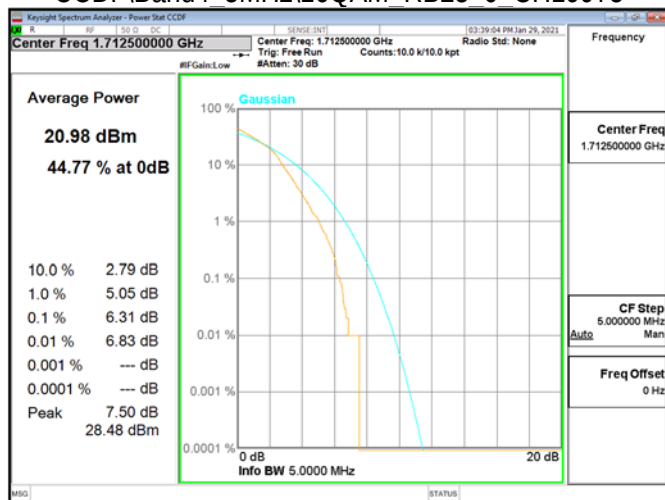
CCDF\Band4 5MHz\16QAM RB25 0 CH19975
