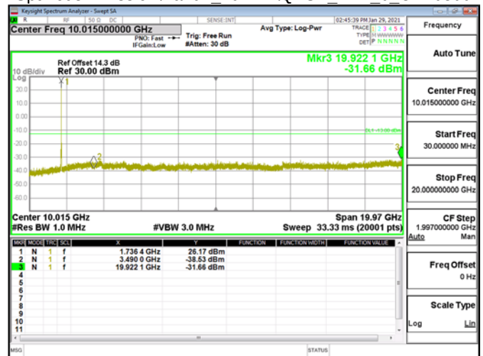
Spurious Emission\Band4 20MHz\QPSK RB1_0_CH20300
