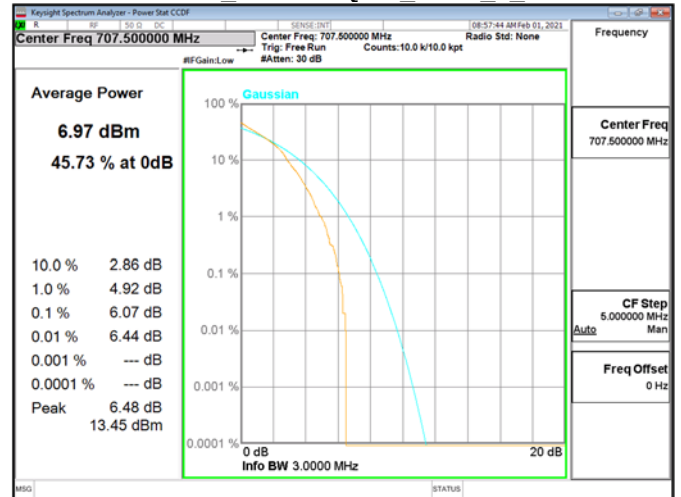
CCDF\Band12 3MHz\16QAM RB15 0 CH23095
