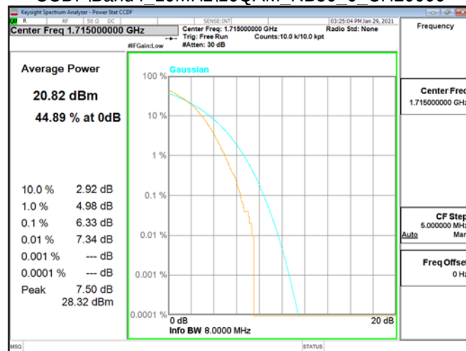
CCDF\Band4 10MHz\16QAM RB50 0 CH20000
