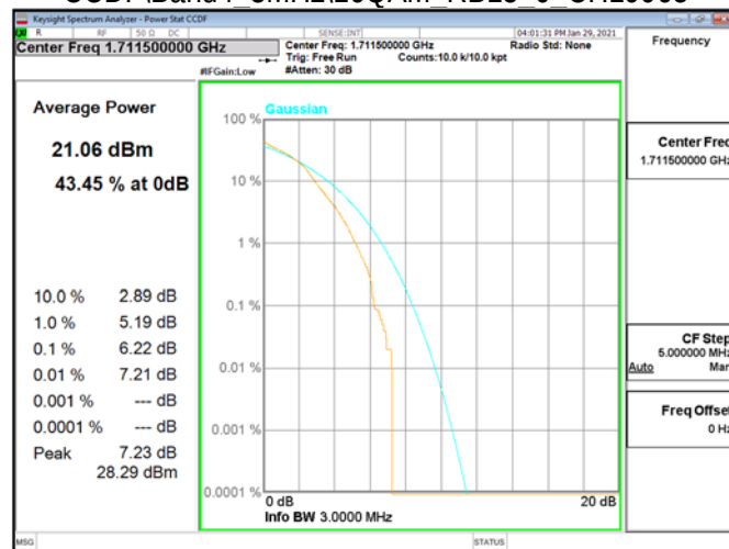
CCDF\Band4 3MHz\16QAM RB15 0 CH19965
