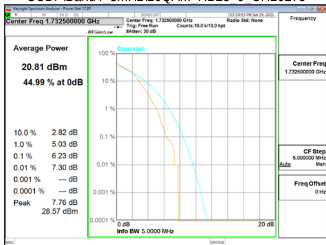
CCDF\Band4 5MHz\16QAM RB25 0 CH20175
