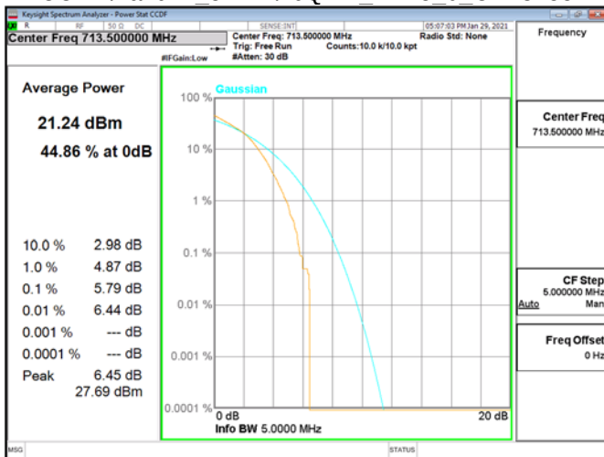
CCDF\Band12 5MHz\16QAM RB25 0 CH23155
