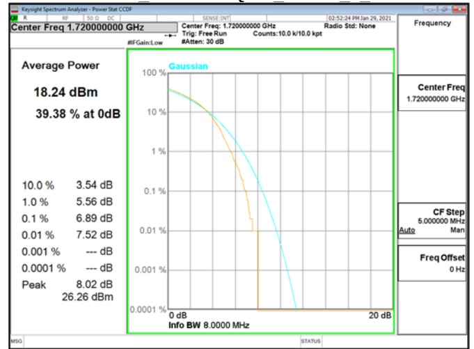
CCDF\Band4 20MHz\16QAM RB100 0 CH20050
