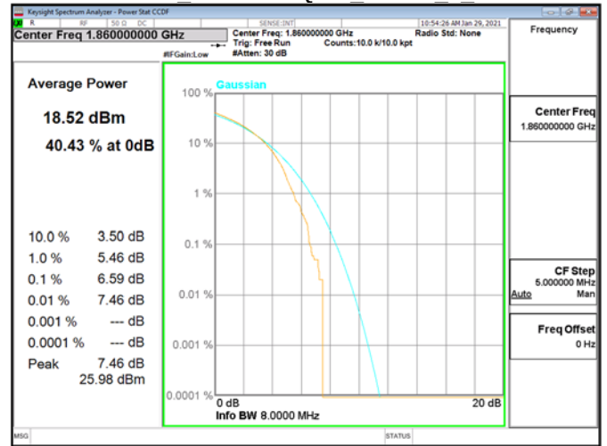
CCDF\Band2 20MHz\16QAM RB100 0 CH18700
