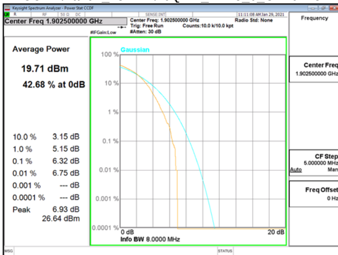
CCDF\Band2 15MHz\16QAM RB75 0 CH19125
