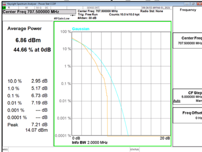
CCDF\Band12 1.4MHz\16QAM RB6 0 CH23095
