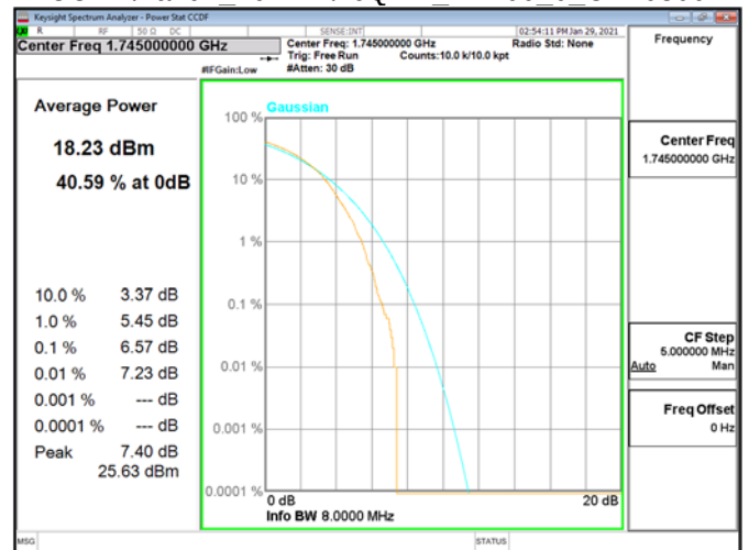
CCDF\Band4 20MHz\16QAM RB100 0 CH20300
