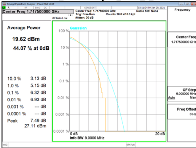
CCDF\Band4 15MHz\16QAM RB75 0 CH20025
