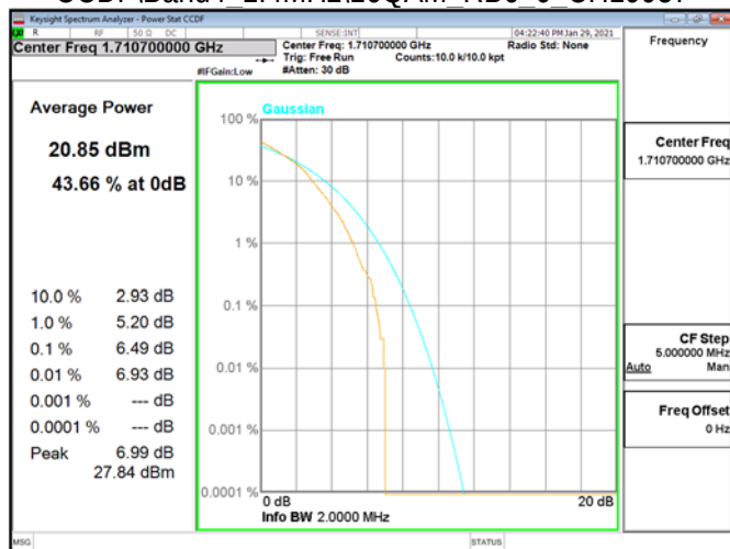
CCDF\Band4 1.4MHz\16QAM RB6 0 CH19957
