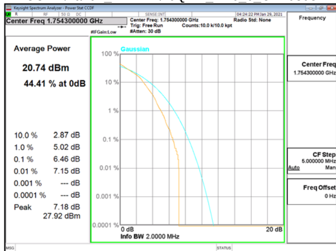
CCDF\Band4 1.4MHz\16QAM RB6 0 CH20393
