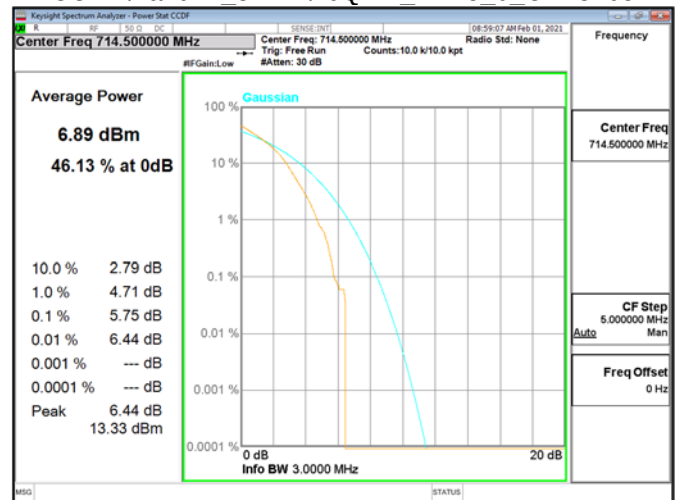
CCDF\Band12 3MHz\16QAM RB15 0 CH23165
