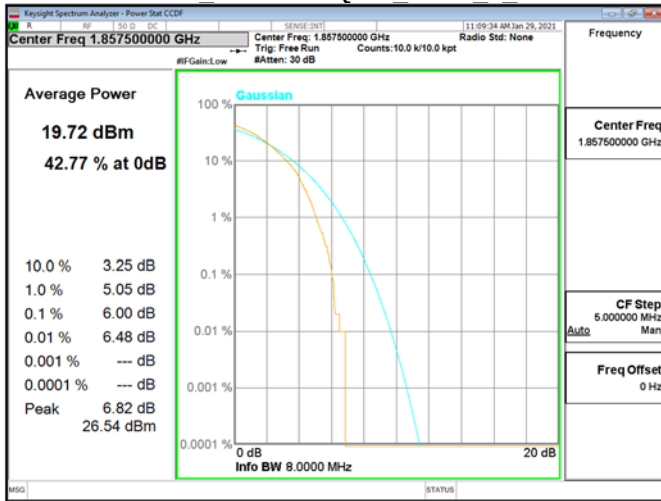
CCDF\Band2 15MHz\16QAM RB75 0 CH18675
