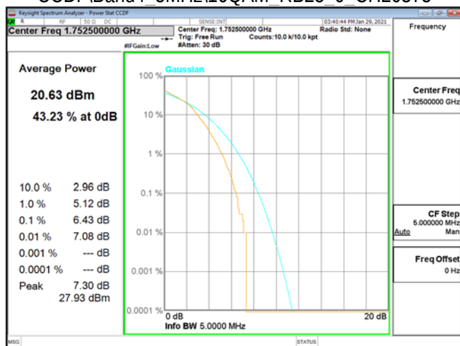
CCDF\Band4 5MHz\16QAM RB25 0 CH20375
