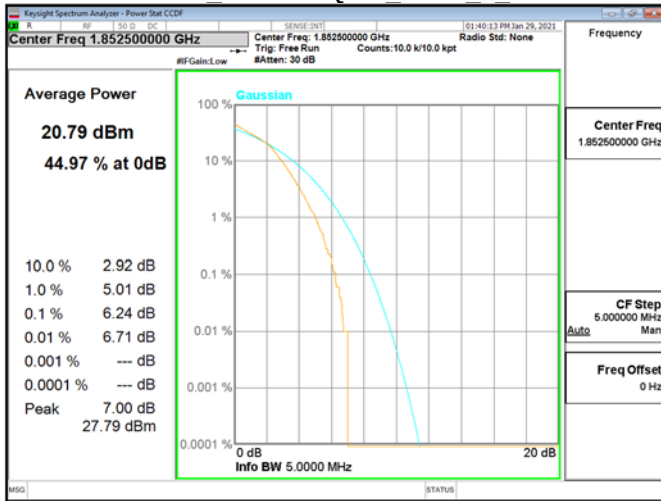
CCDF\Band2 5MHz\16QAM RB25 0 CH18625
