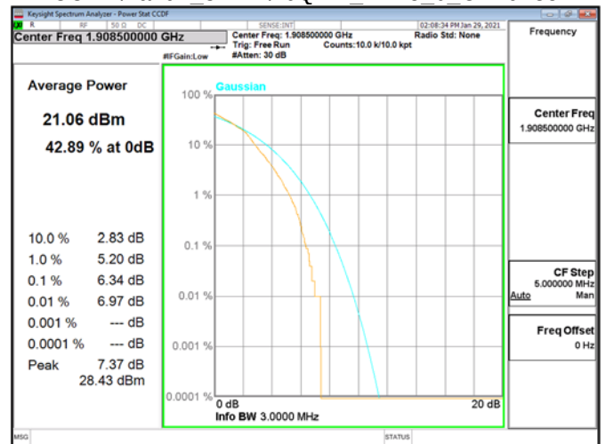
CCDF\Band2 3MHz\16QAM RB15 0 CH19185
