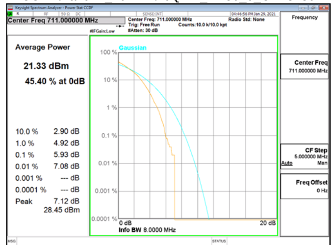
CCDF\Band12 10MHz\16QAM RB50 0 CH23130
