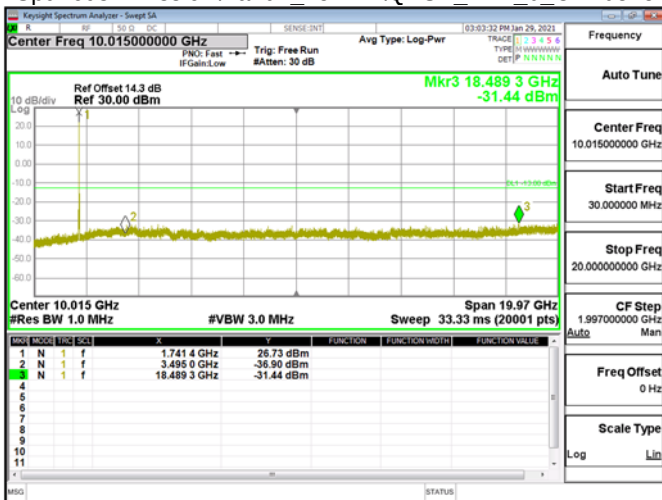
Spurious Emission\Band4 15MHz\QPSK RB1_0_CH20325
