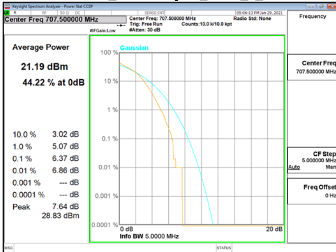
CCDF\Band12 5MHz\16QAM RB25 0 CH23095
