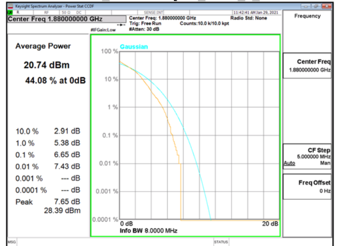
CCDF\Band2 10MHz\16QAM RB50 0 CH18900
