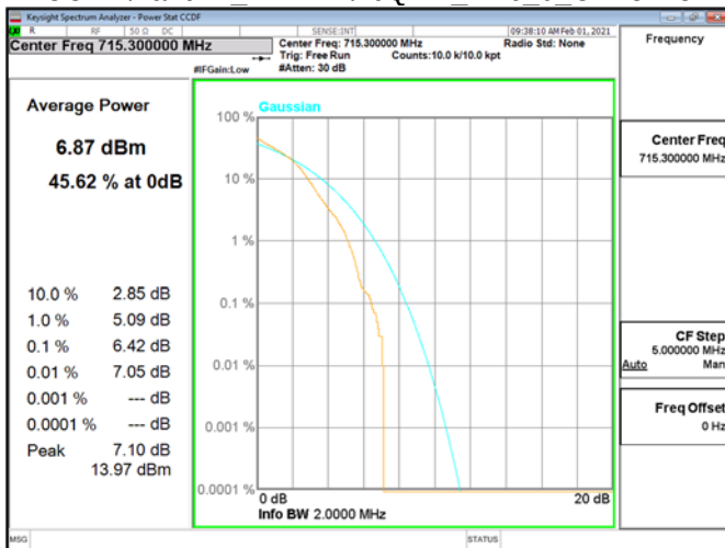
CCDF\Band12 1.4MHz\16QAM RB6 0 CH23173
