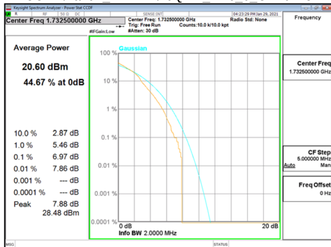
CCDF\Band4 1.4MHz\16QAM RB6 0 CH20175
