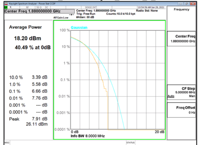
CCDF\Band2 20MHz\16QAM RB100 0 CH18900
