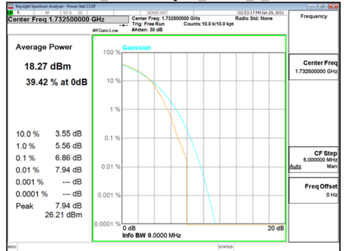
CCDF\Band4 20MHz\16QAM RB100 0 CH20175
