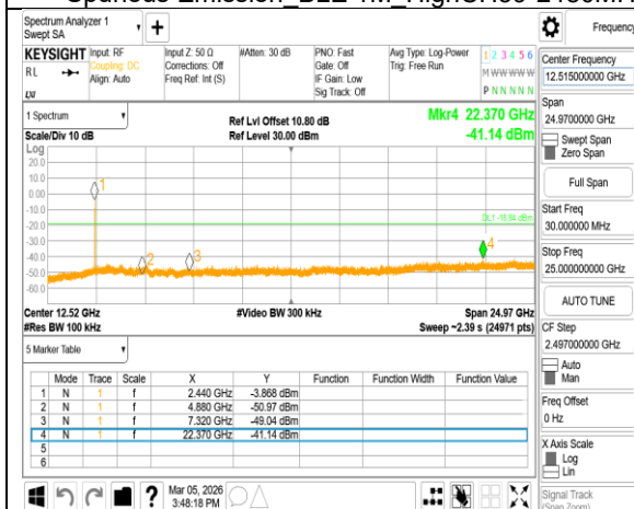
Spurious Emission_BLE 2M_MidCH19-2440MHz
