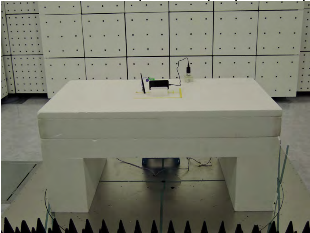
Radiated Emission Set up Photos E1 plan (Below 1GHz)
