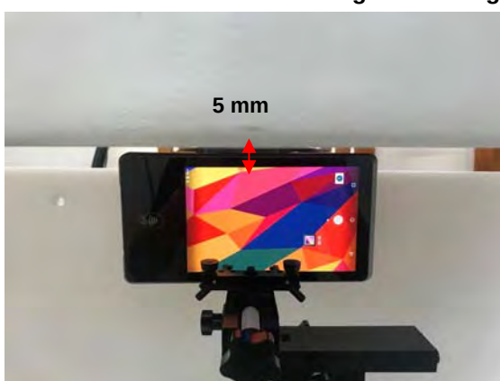
Fig.15 EUT Left side to flat phantom
