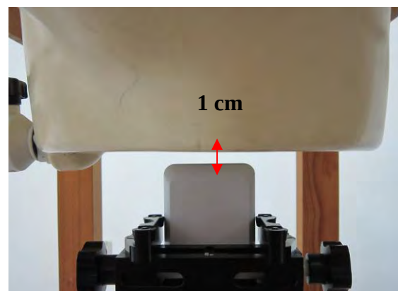
Fig.5 EUT Left to flat phantom
