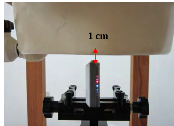
Fig.4 EUT Bottom to flat phantom
