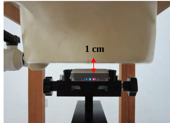
Fig.7 EUT Back to flat phantom
