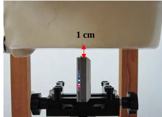
Fig.3 EUT Top to flat phantom
