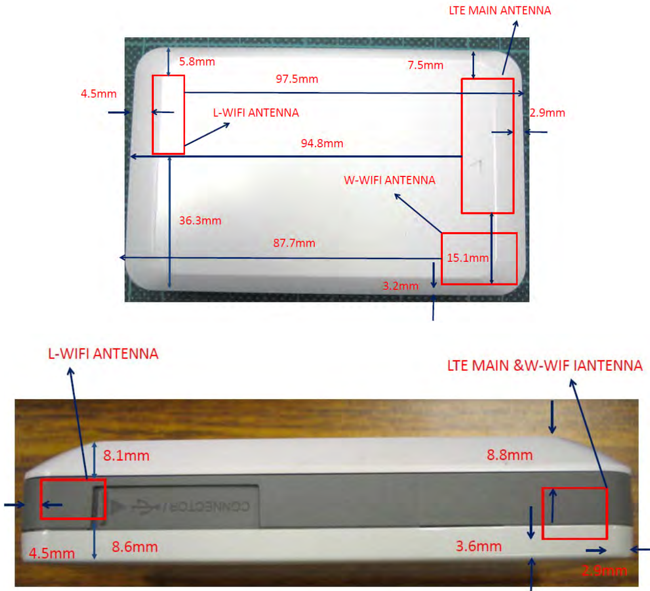
Fig.12 Antenna position of EUT
