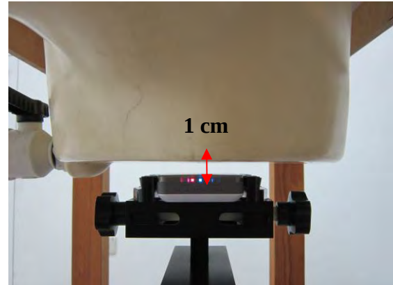
Fig.6 EUT Front to flat phantom
