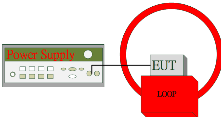
Fig. 2-1 Conducted Emission
