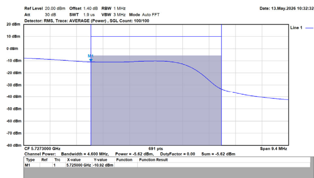
802.11ac/20MHz/MCS0/5720MHz/Ch144/Ant.1 (UNII-3)
