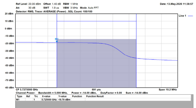
802.11ac/80MHz/MCS0/5690MHz/Ch138/Ant.2 (UNII-3)
