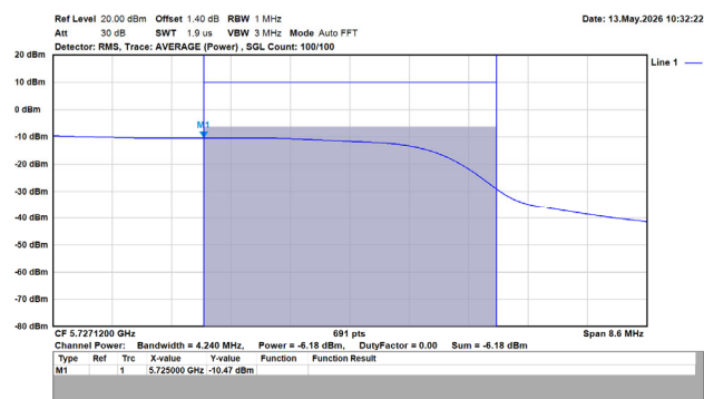
802.11a/20MHz/6M/5720MHz/Ch144/Ant.2 (UNII-3)
