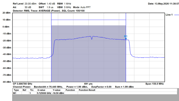
802.11ac/80MHz/MCS0/5690MHz/Ch138/Ant.2 (UNII-2C)
