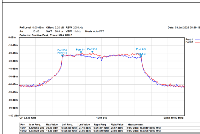
802.11ax/20MHz/MCS0/6535MHz/Ch117 (OBW)
