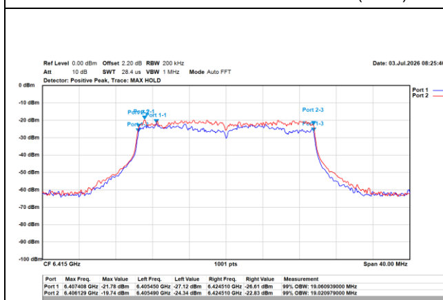
802.11ax/20MHz/MCS0/6415MHz/Ch93 (OBW)
