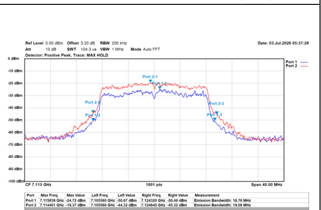
802.11a/20MHz/6M/7115MHz/Ch233 (EBW)
