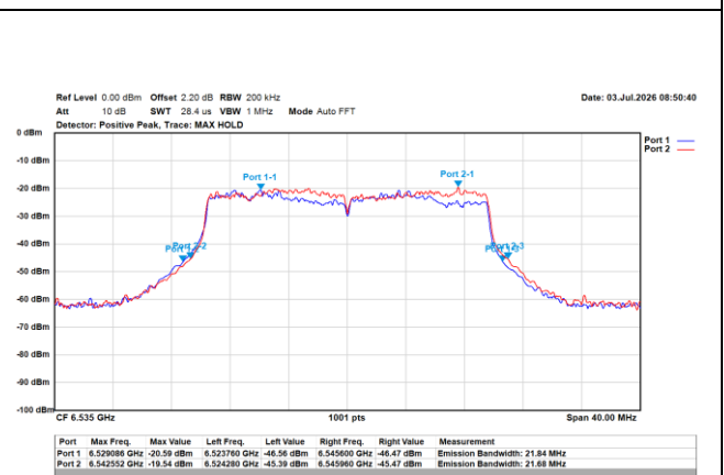
802.11ax/20MHz/MCS0/6535MHz/Ch117 (EBW)
