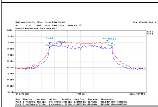
802.11ax/20MHz/MCS0/6175MHz/Ch45 (OBW)
