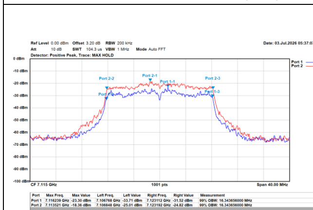
802.11a/20MHz/6M/7115MHz/Ch233 (OBW)
