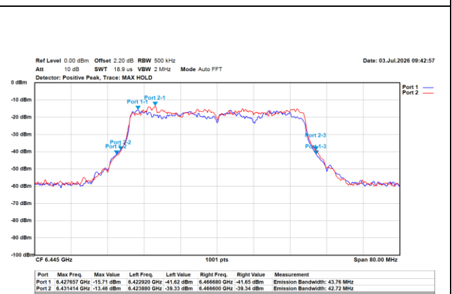
802.11ax/40MHz/MCS0/6445MHz/Ch99 (EBW)
