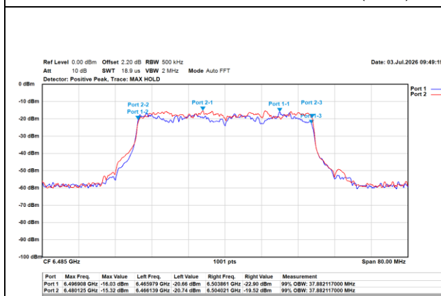
802.11ax/40MHz/MCS0/6485MHz/Ch107 (OBW)
