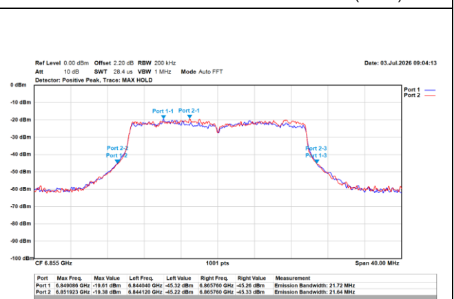
802.11ax/20MHz/MCS0/6855MHz/Ch181 (EBW)
