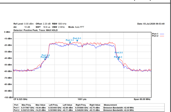
802.11ax/40MHz/MCS0/6525MHz/Ch115 (EBW)
