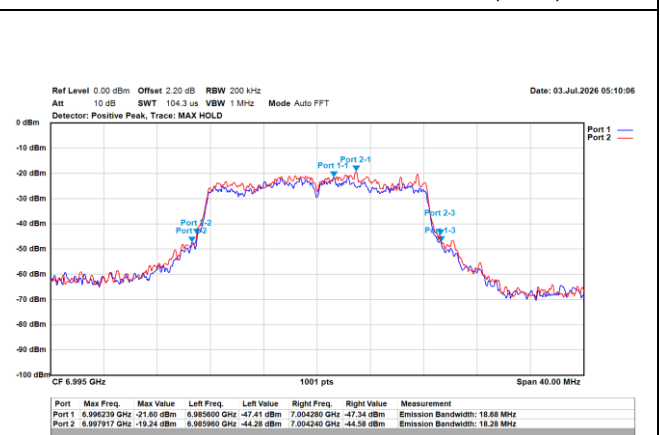
802.11a/20MHz/6M/6995MHz/Ch209 (EBW)
