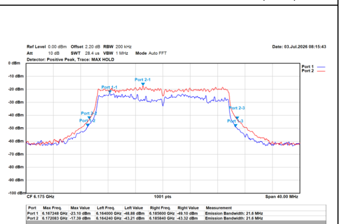
802.11ax/20MHz/MCS0/6175MHz/Ch45 (EBW)
