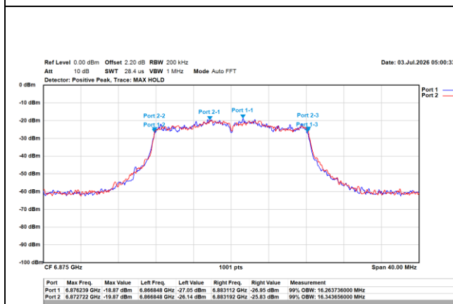
802.11a/20MHz/6M/6875MHz/Ch185 (OBW)
