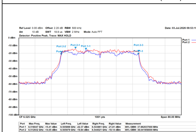
802.11ax/40MHz/MCS0/6525MHz/Ch115 (OBW)
