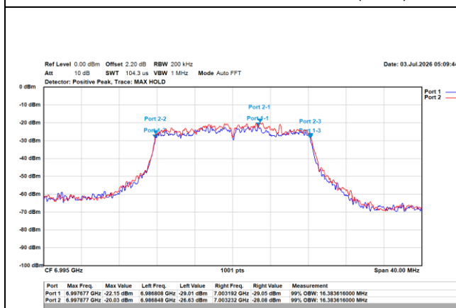
802.11a/20MHz/6M/6995MHz/Ch209 (OBW)
