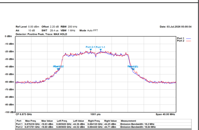
802.11a/20MHz/6M/6875MHz/Ch185 (EBW)
