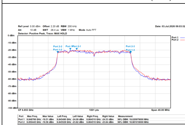
802.11ax/20MHz/MCS0/6855MHz/Ch181 (OBW)
