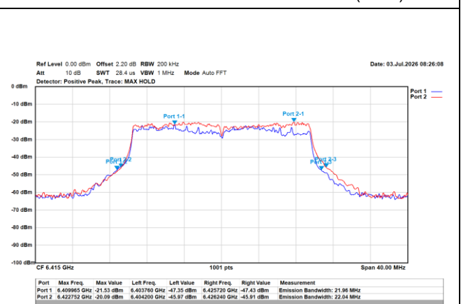
802.11ax/20MHz/MCS0/6415MHz/Ch93 (EBW)
