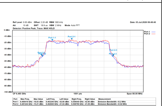
802.11ax/40MHz/MCS0/6485MHz/Ch107 (EBW)
