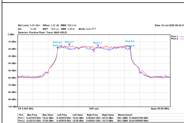
802.11ax/40MHz/MCS0/6445MHz/Ch99 (OBW)
