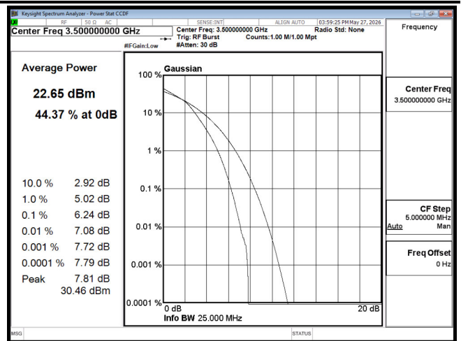
PTAR B42 20M CH42590 16QAM
