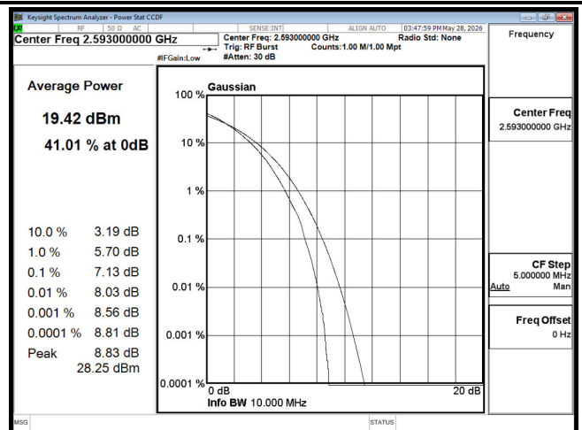
PTAR B41 10M CH40620 256QAM
