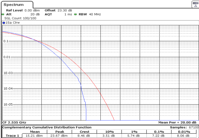
PTAR B7 15M CH21025(75,0),15M CH21175(75,0) 16QAM
