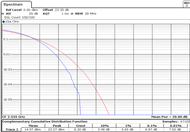
PTAR B7 15M CH21051(75,0),10M CH21171(50,0) 256QAM
