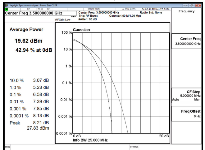
PTAR B42 20M CH42590 256QAM
