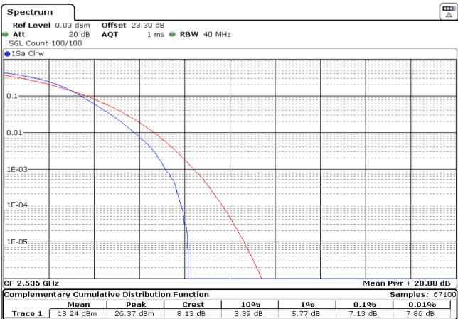
PTAR B7 15M CH21051(75,0),10M CH21171(50,0) 64QAM
