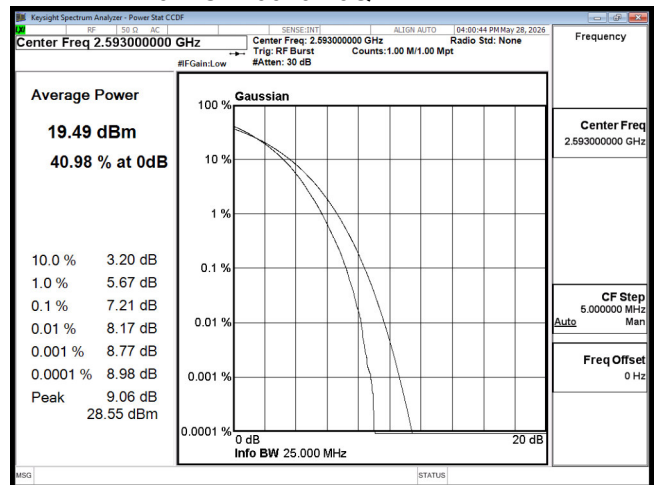
PTAR B41 20M CH40620 256QAM
