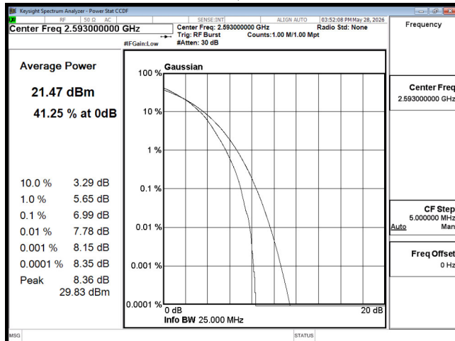
PTAR B41 15M CH40620 64QAM
