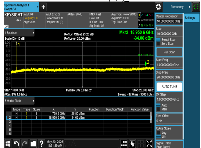
CSE B4 5M CH19975 QPSK(1,0)
