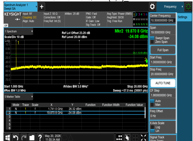
CSE B4 15M CH20325 QPSK(1,0)_
