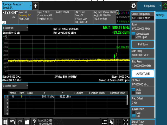
CSE B4 3M CH20385 QPSK(1,0)
