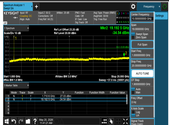
CSE B4 10M CH20000 QPSK(1,0)
