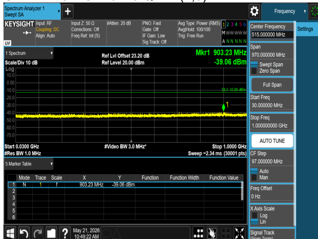
CSE B4 10M CH20350 QPSK(1,0)
