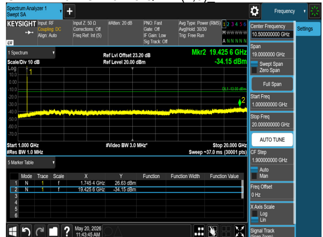
CSE B4 10M CH20350 QPSK(1,0)_
