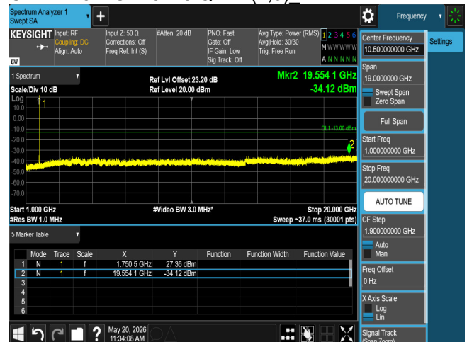
CSE B4 5M CH20175 QPSK(1,0)_
