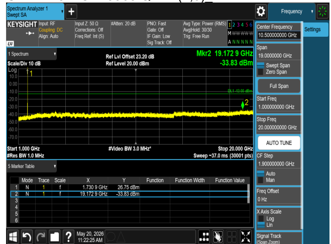
CSE B4 3M CH20175 QPSK(1,0)
