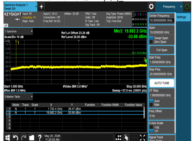
CSE B4 3M CH20385 QPSK(1,0)
