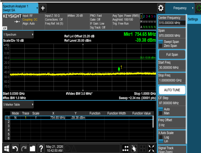
CSE B4 15M CH20025 QPSK(1,0)
