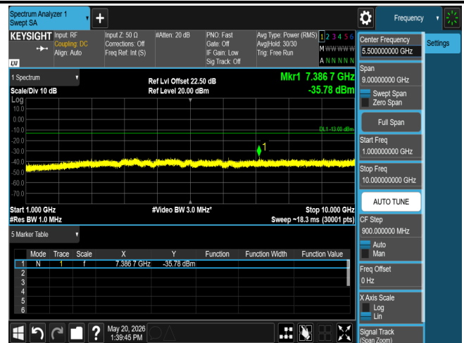
CSE B26 3M CH26805 QPSK(1,0)
