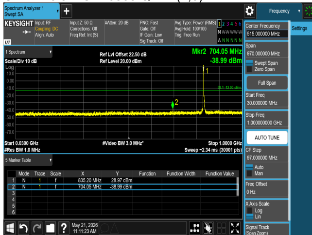
CSE B26 3M CH26805 QPSK(1,0)
