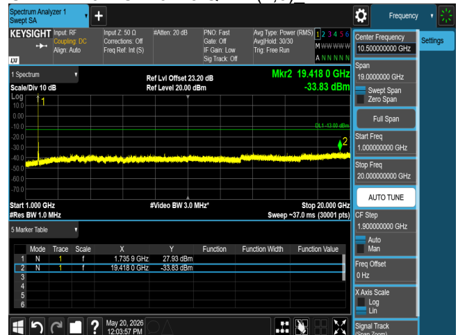
CSE B4 20M CH20300 QPSK(1,0)_
