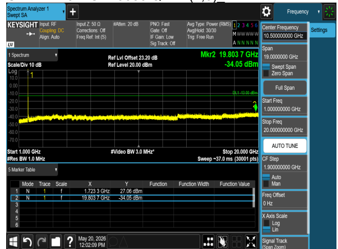
CSE B4 20M CH20175 QPSK(1,0)
