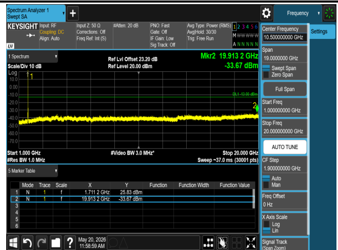
CSE B4 20M CH20050 QPSK(1,0)
