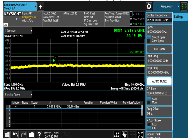
CSE B26 3M CH26775 QPSK(1,0)_
