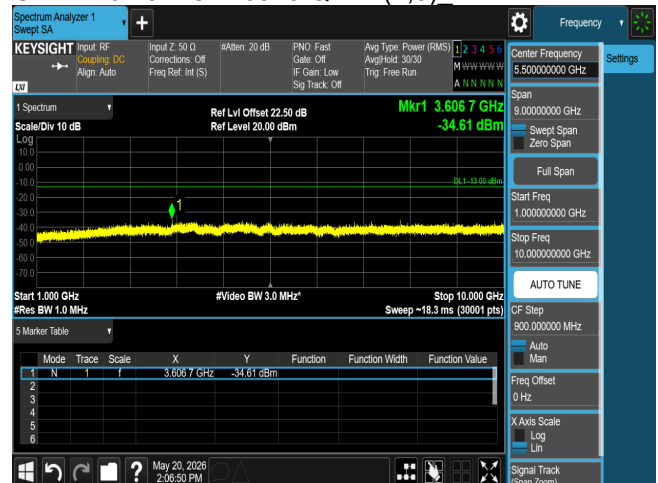
CSE B26 10M CH26990 QPSK(1,0)_
