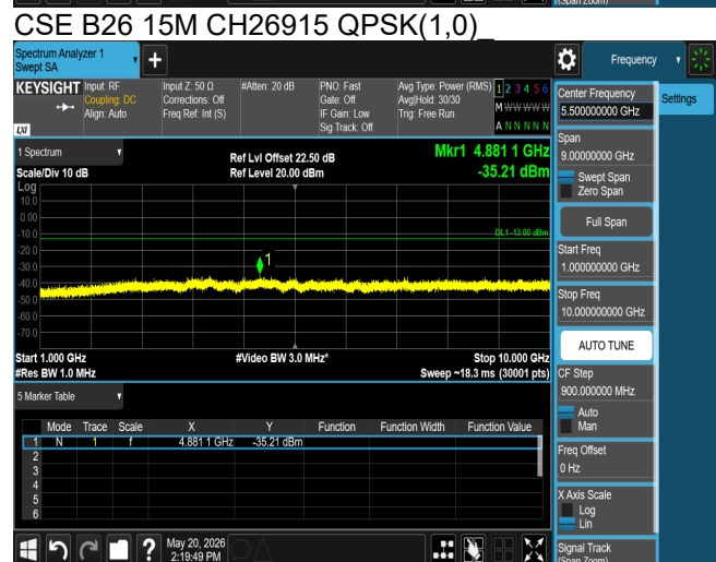
CSE B26 15M CH26915 QPSK(1,0)_
