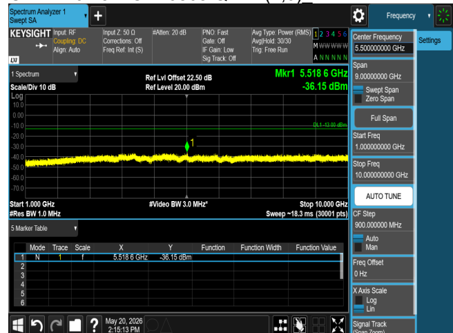
CSE B26 15M CH26865 QPSK(1,0)
