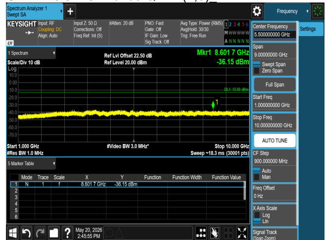
CSE B26 3M CH26740 QPSK(1,0)
