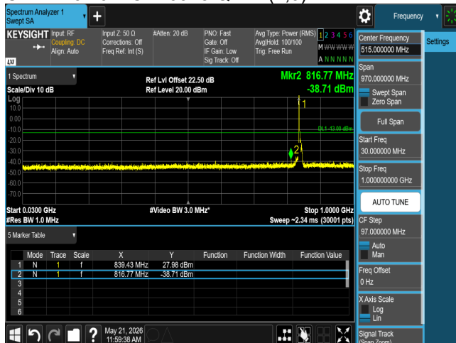
CSE B26 10M CH26990 QPSK(1,0)
