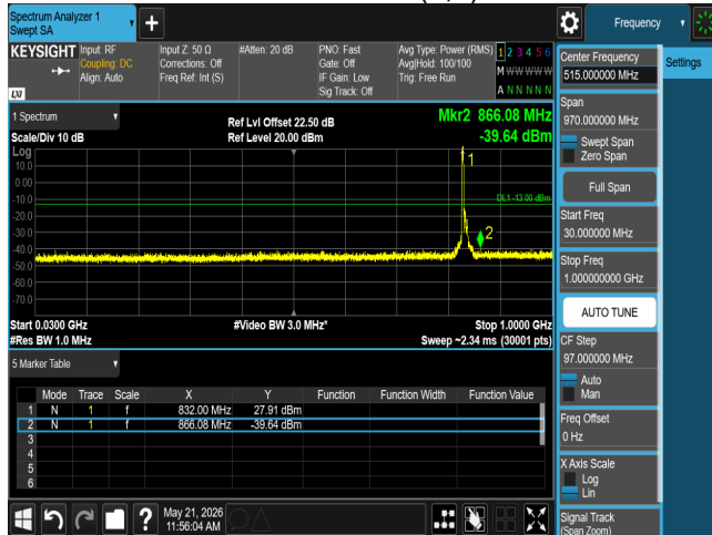
CSE B26 10M CH26915 QPSK(1,0)
