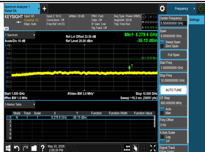
CSE B26 15M CH26865 QPSK(1,0)
