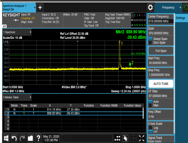
CSE B26 5M CH26715 QPSK(1,0)
