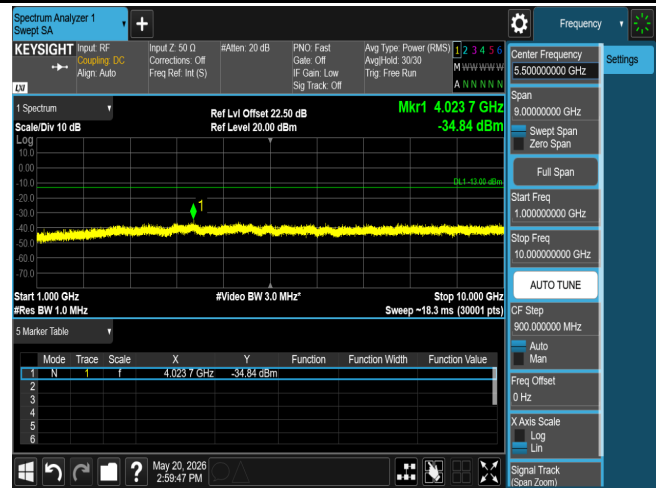
CSE B26 10M CH26740 QPSK(1,0)_
