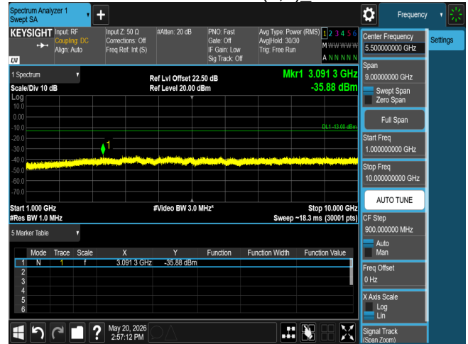
CSE B26 5M CH26715 QPSK(1,0)
