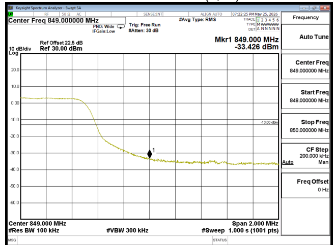
EDGE B26 10M CH26990 QPSK(50,0)
