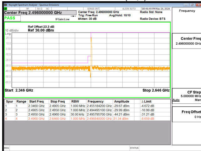
EDGE B41 15M CH39725 QPSK(1,0)
