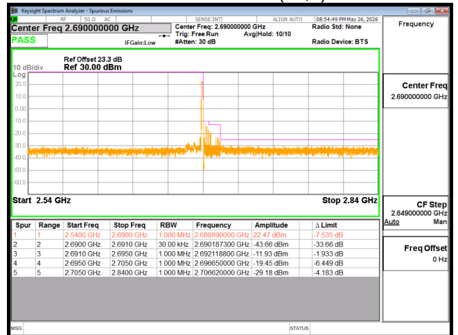
EDGE B41 15M CH41515 QPSK(1,74)
