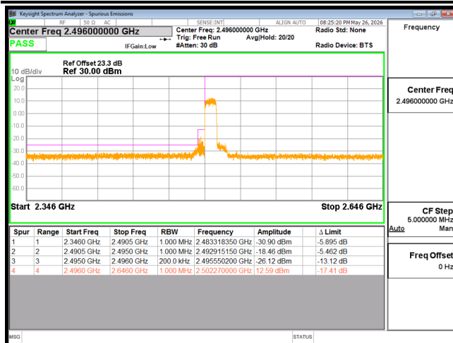
EDGE B41 10M CH39700 QPSK(50,0)
