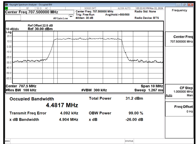
OCC B12 5M CH23095 256QAM
