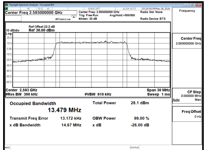
OCC B41 15M CH40620 256QAM
