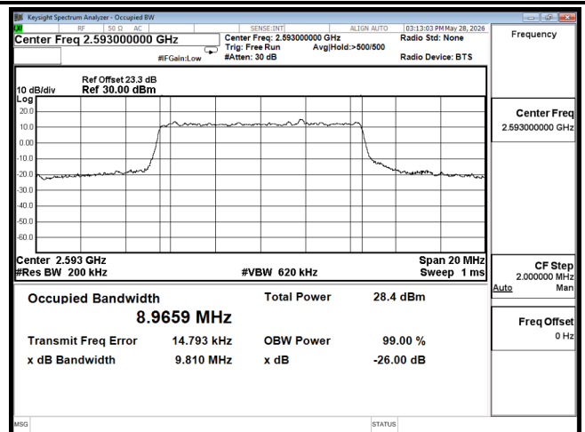
OCC B41 10M CH40620 256QAM
