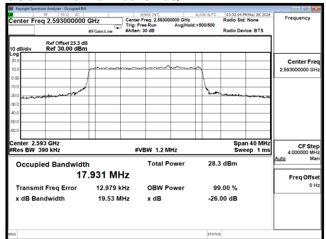
OCC B41 20M CH40620 256QAM
