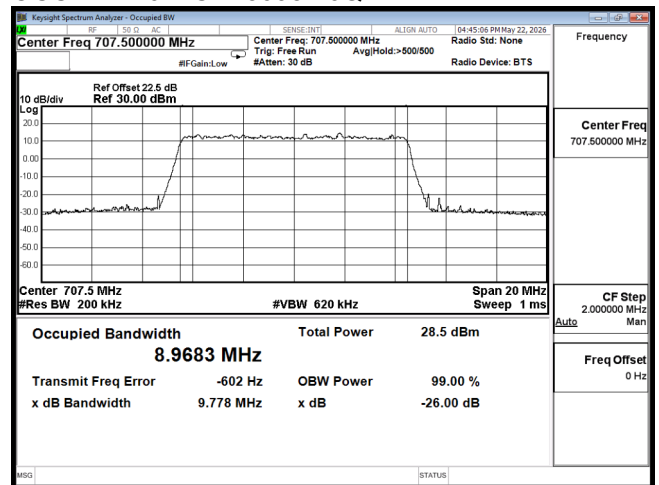
OCC B12 10M CH23095 256QAM
