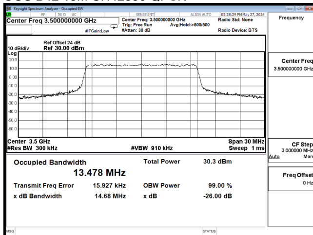
OCC B42 15M CH42590 64QAM
