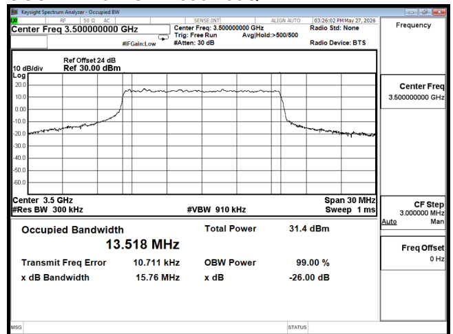
OCC B42 15M CH42590 16QAM
