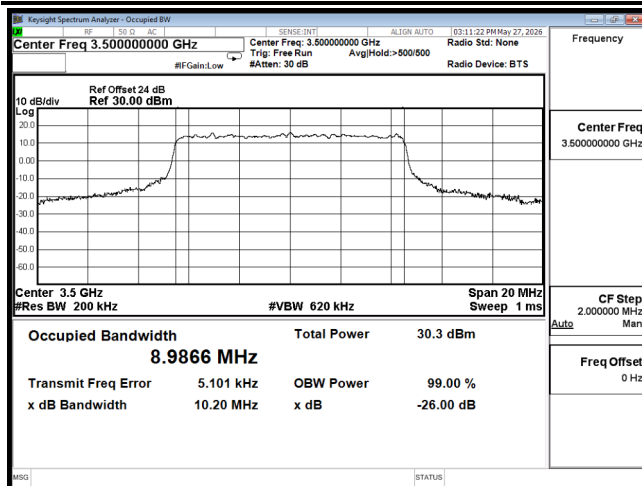
OCC B42 10M CH42590 64QAM
