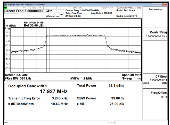
OCC B42 20M CH42590 256QAM
