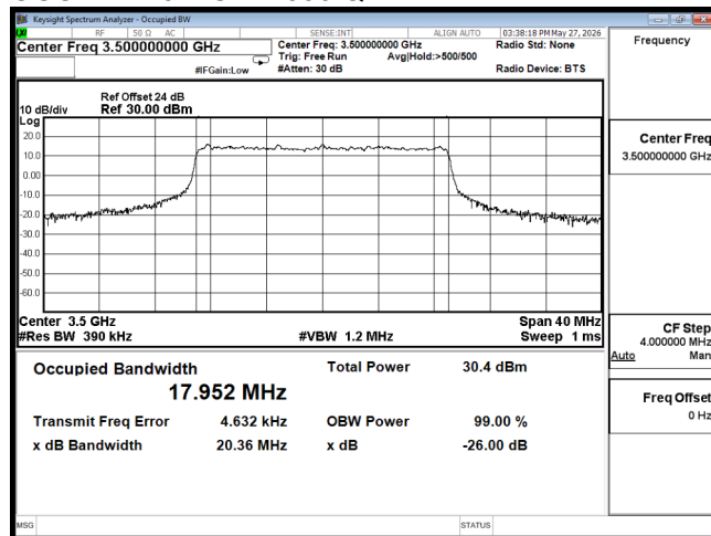
OCC B42 20M CH42590 64QAM
