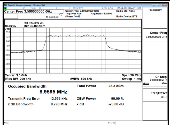
OCC B42 10M CH42590 256QAM
