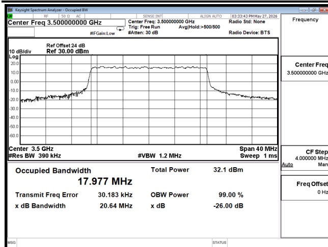
OCC B42 20M CH42590 QPSK
