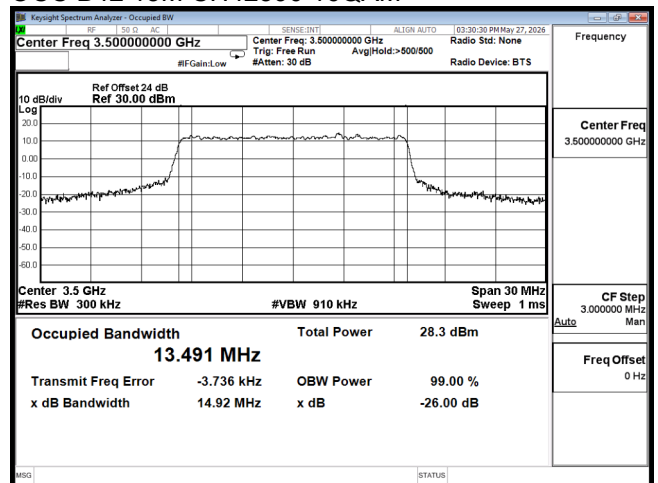
OCC B42 15M CH42590 256QAM
