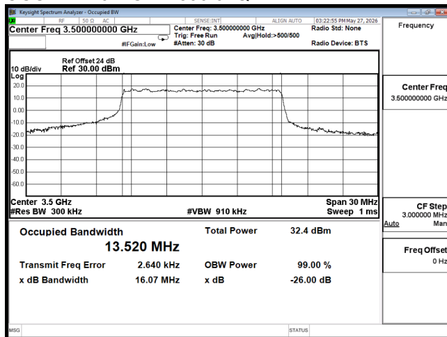
OCC B42 15M CH42590 QPSK
