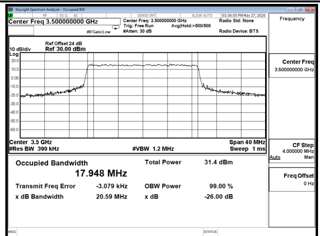
OCC B42 20M CH42590 16QAM
