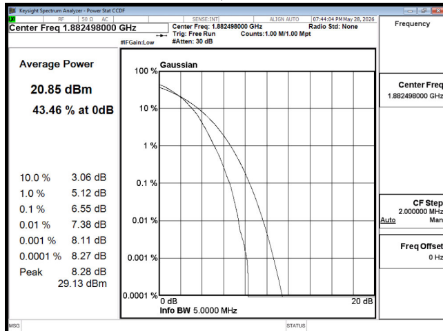
PTAR B25 5M CH26365 64QAM
