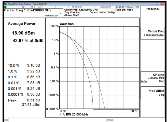
PTAR B25 20M CH26365 256QAM
