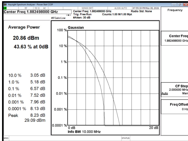
PTAR B25 10M CH26365 64QAM
