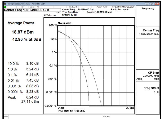
PTAR B25 10M CH26365 256QAM
