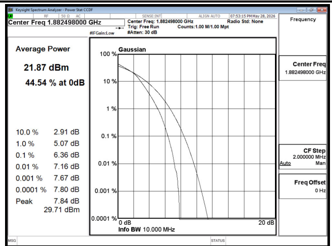
PTAR B25 10M CH26365 16QAM
