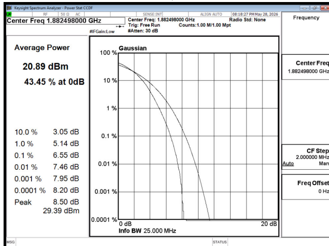
PTAR B25 20M CH26365 64QAM
