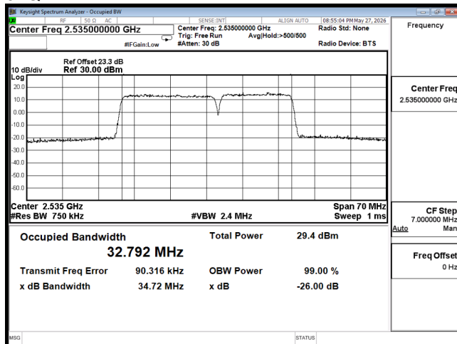
OCC B7 20M CH21026(100,0),15M CH21197(75,0) QPSK
