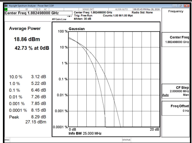
PTAR B25 15M CH26365 256QAM
