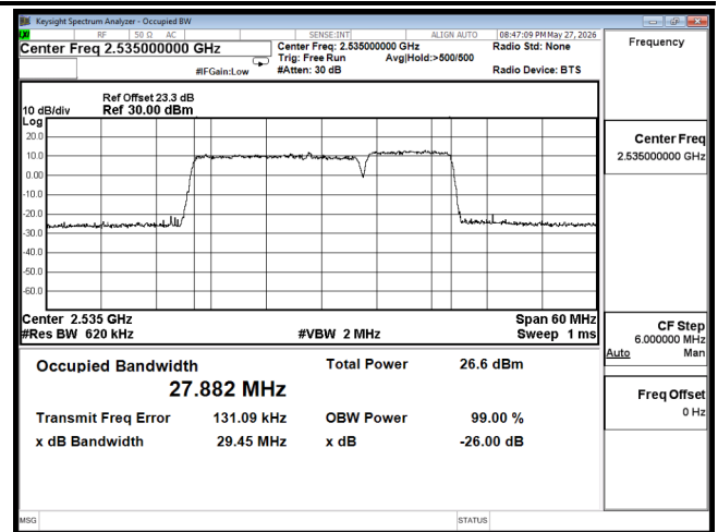
OCC B7 20M CH21051(100,0),10M CH21195(50,0) 256QAM
