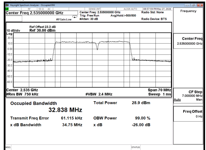
OCC B7 20M CH21026(100,0),15M CH21197(75,0) 256QAM
