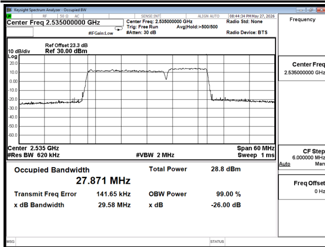
OCC B7 20M CH21051(100,0),10M CH21195(50,0) 64QAM
