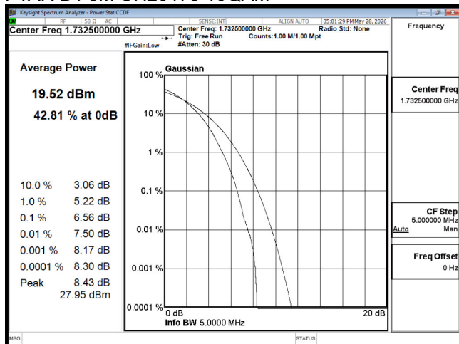
PTAR B4 5M CH20175 256QAM
