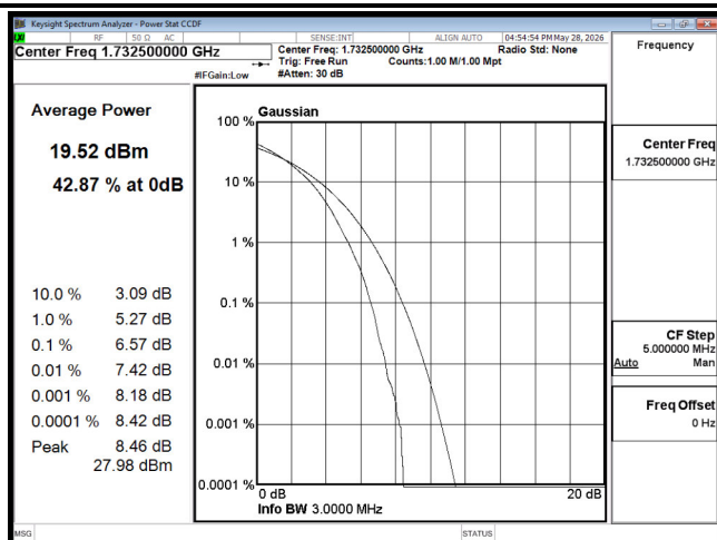
PTAR B4 3M CH20175 256QAM
