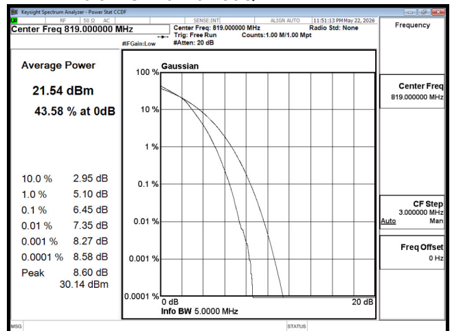
PTAR B26 5M CH26740 16QAM
