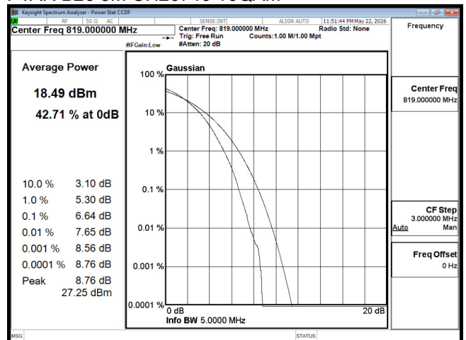
PTAR B26 5M CH26740 256QAM
