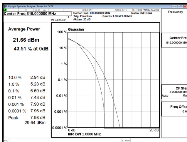
PTAR B26 1.4M CH26740 16QAM
