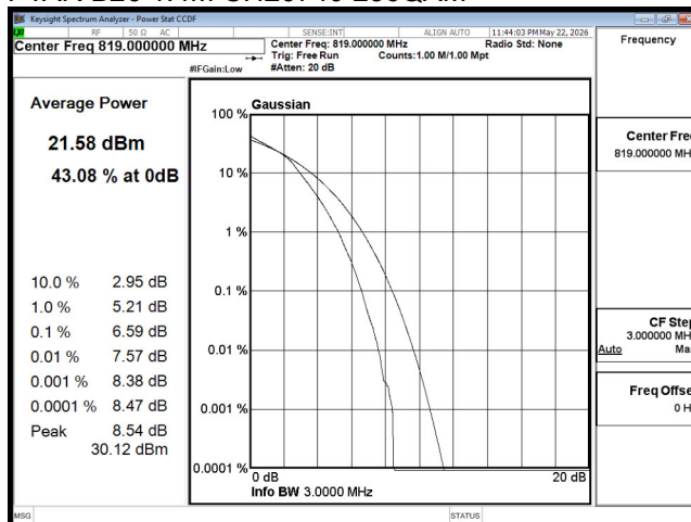
PTAR B26 3M CH26740 16QAM
