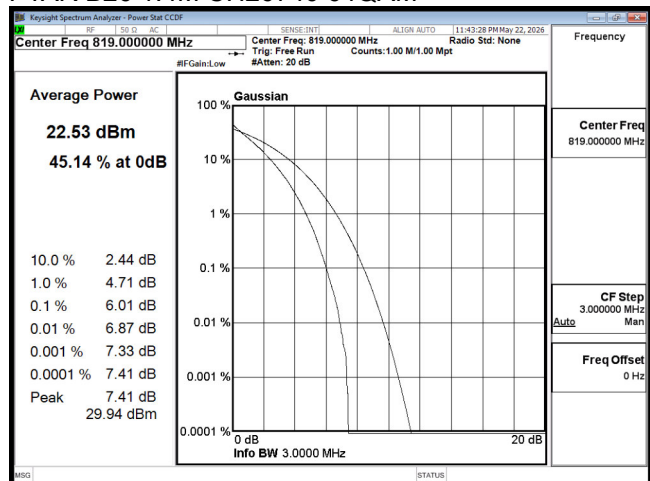
PTAR B26 3M CH26740 QPSK
