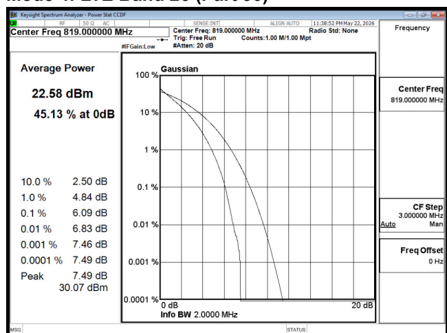
PTAR B26 1.4M CH26740 QPSK
