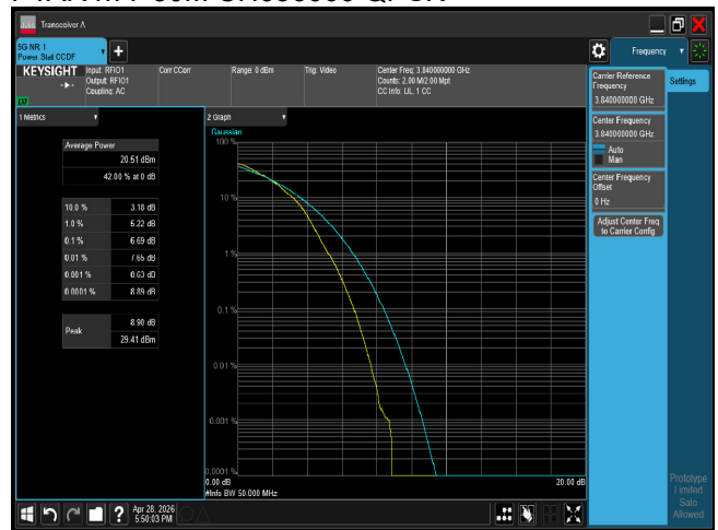
PTAR n77 50M CH656000 64QAM
