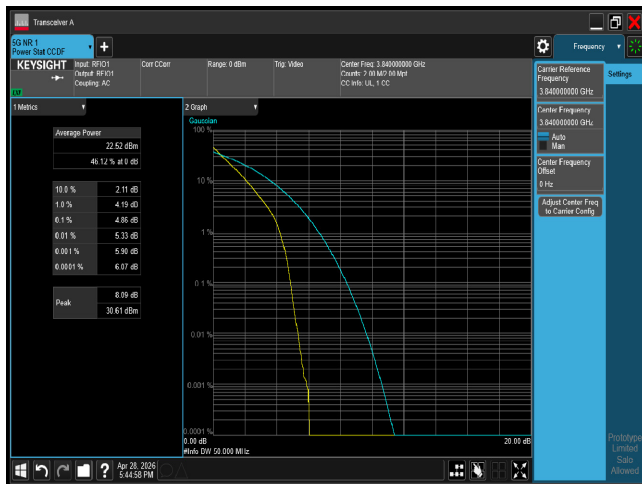
PTAR n77 50M CH656000 BPSK
