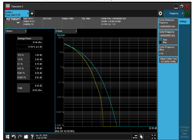
PTAR n77 40M CH656000 256QAM
