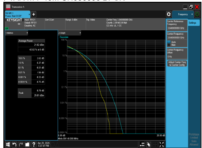
PTAR n77 40M CH656000 16QAM
