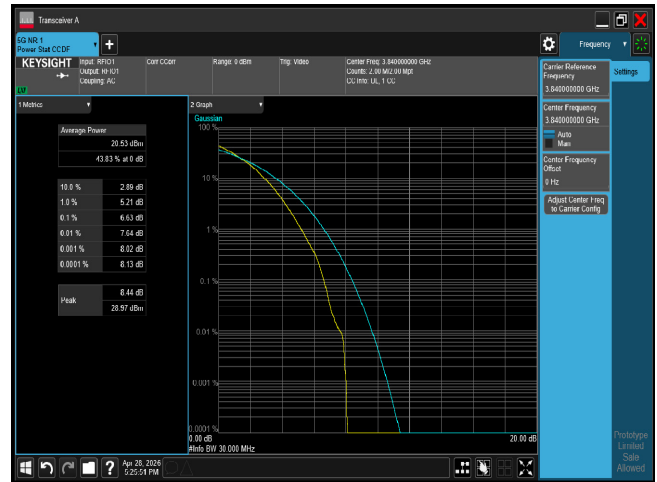
PTAR n77 30M CH656000 64QAM
