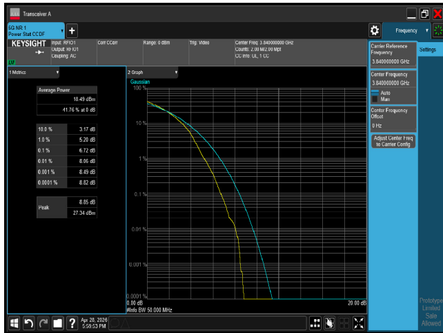
PTAR n77 50M CH656000 256QAM
