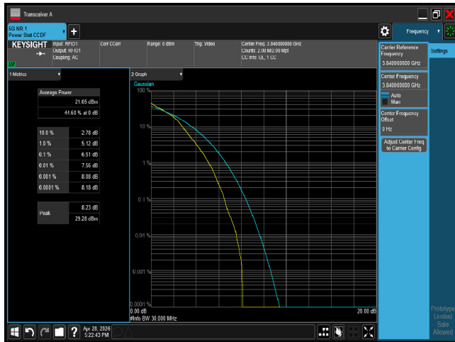
PTAR n77 30M CH656000 16QAM
