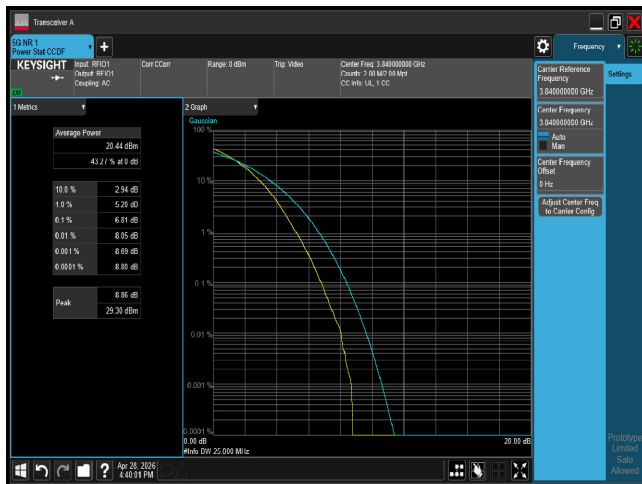
PTAR n77 25M CH656000 64QAM
