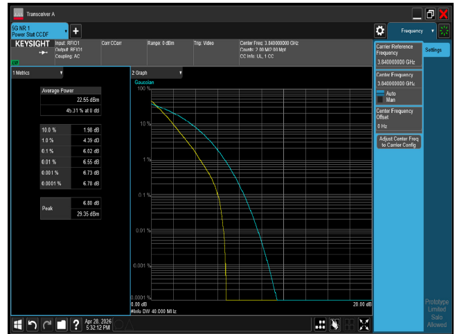
PTAR n77 40M CH656000 BPSK
