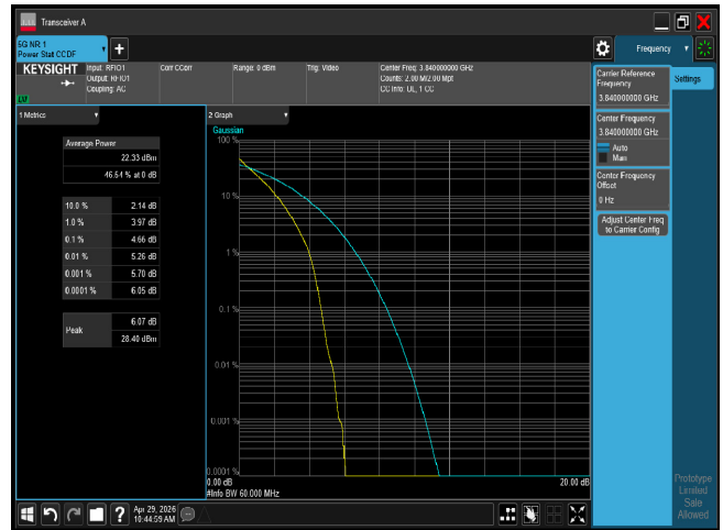
PTAR n77 60M CH656000 BPSK
