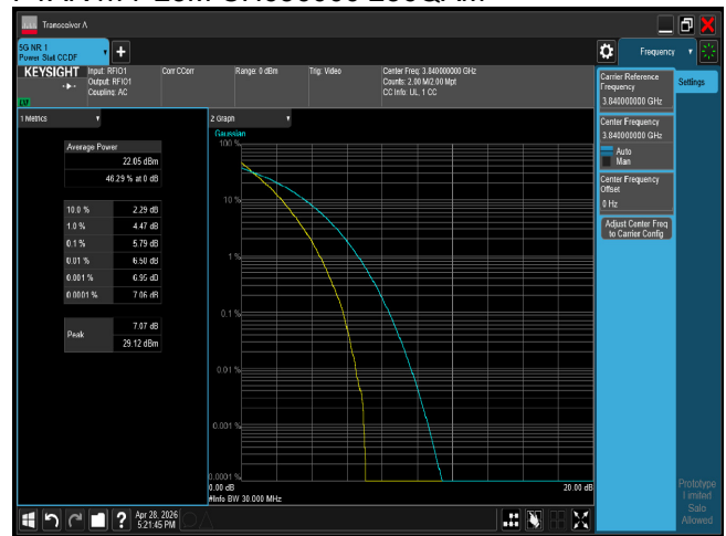
PTAR n77 30M CH656000 QPSK
