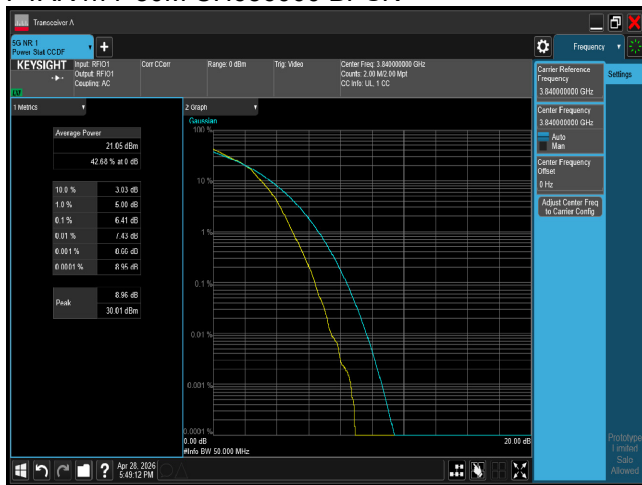
PTAR n77 50M CH656000 16QAM
