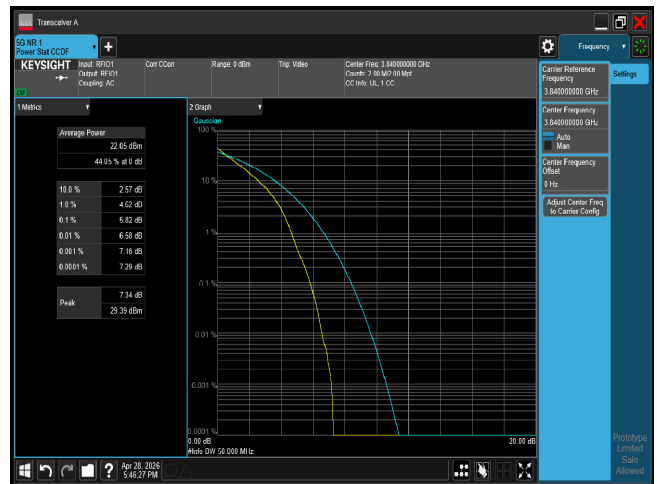
PTAR n77 50M CH656000 QPSK
