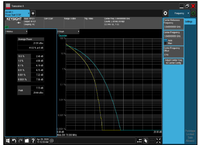
PTAR n77 70M CH656000 QPSK
