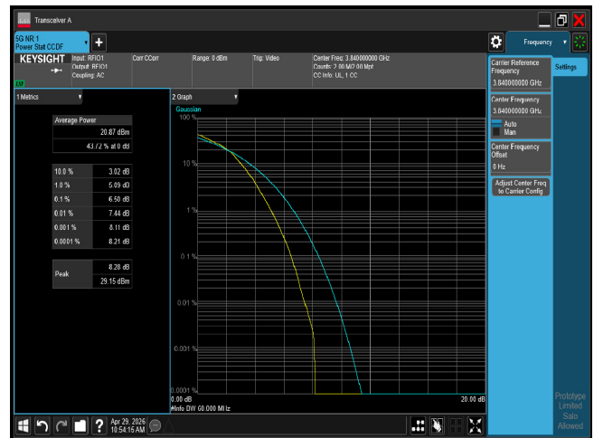
PTAR n77 60M CH656000 16QAM
