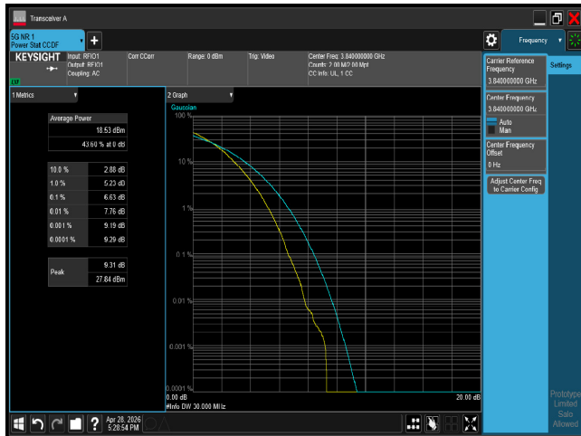
PTAR n77 30M CH656000 256QAM
