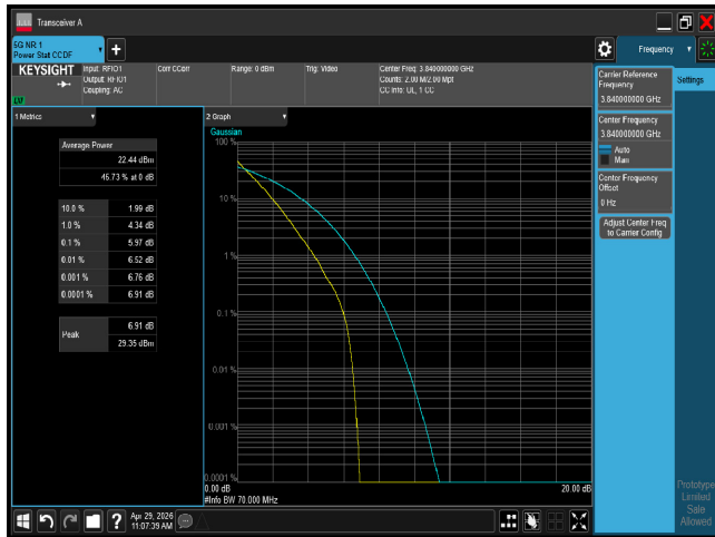
PTAR n77 70M CH656000 BPSK
