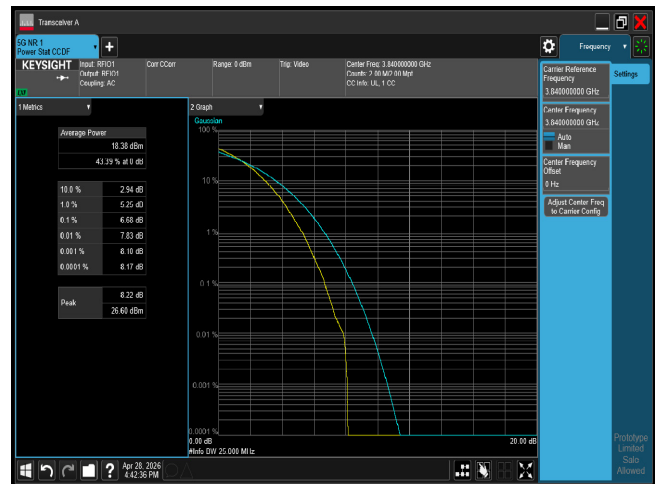
PTAR n77 25M CH656000 256QAM
