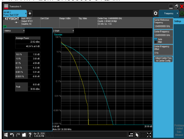
PTAR n77 30M CH656000 BPSK
