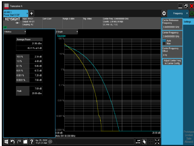
PTAR n77 80M CH656000 QPSK
