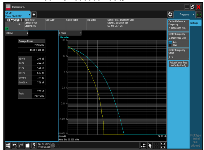
PTAR n77 90M CH656000 QPSK
