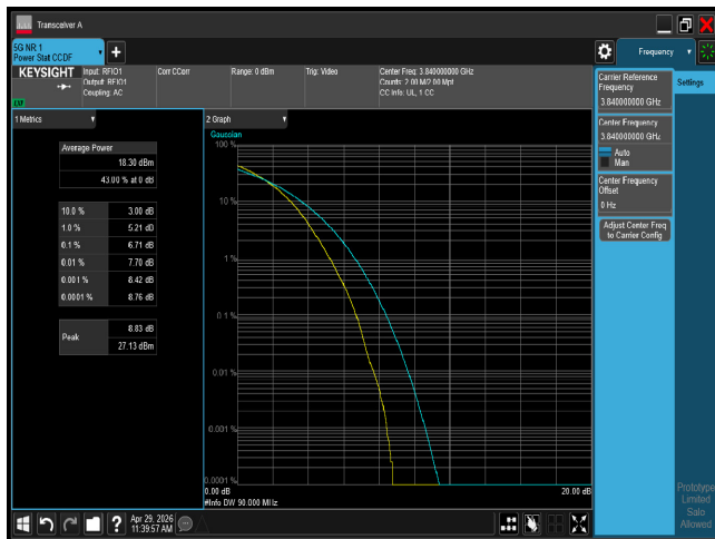
PTAR n77 90M CH656000 256QAM
