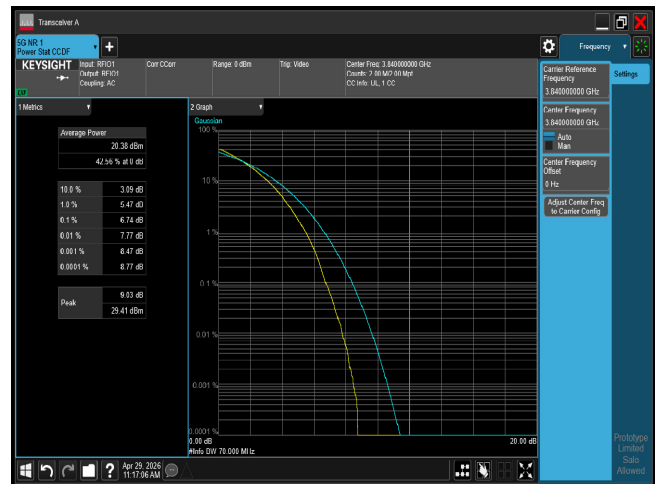
PTAR n77 70M CH656000 64QAM
