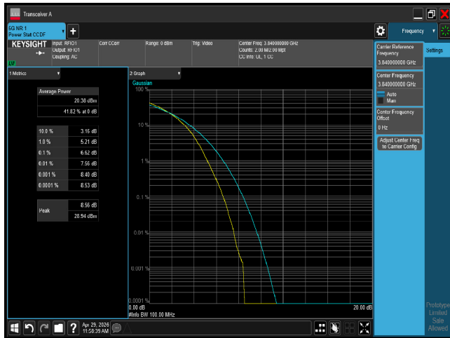
PTAR n77 100M CH656000 64QAM
