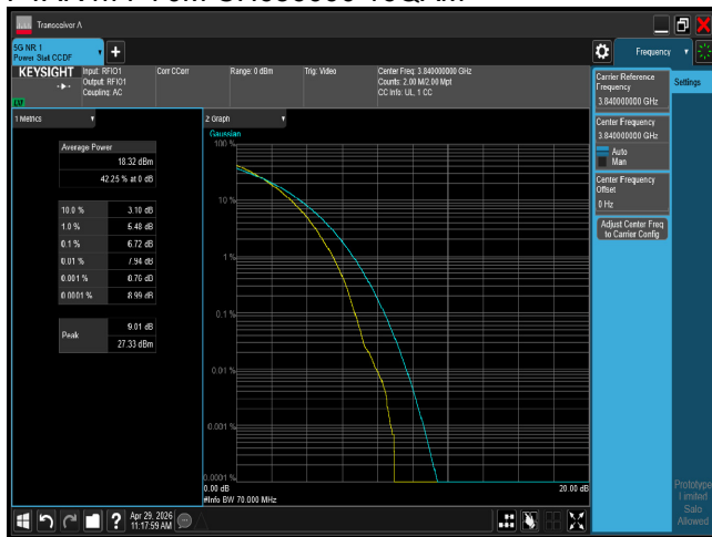
PTAR n77 70M CH656000 256QAM
