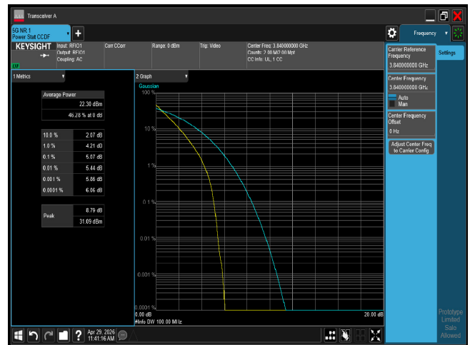
PTAR n77 100M CH656000 BPSK
