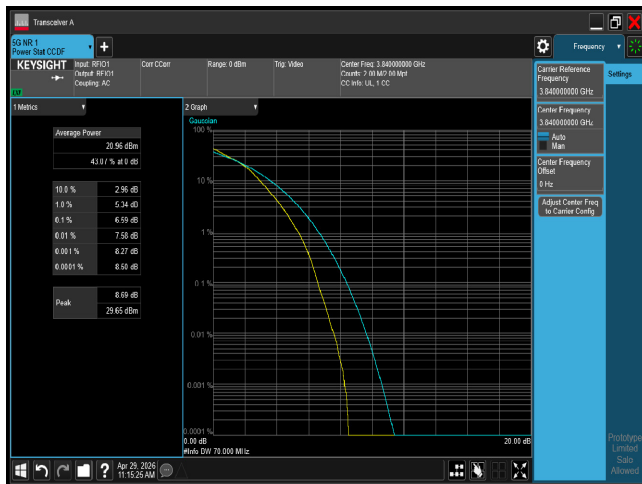
PTAR n77 70M CH656000 16QAM
