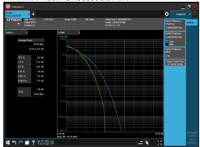
PTAR n77 100M CH656000 16QAM
