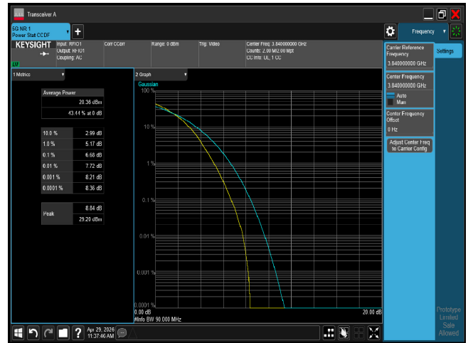
PTAR n77 90M CH656000 64QAM
