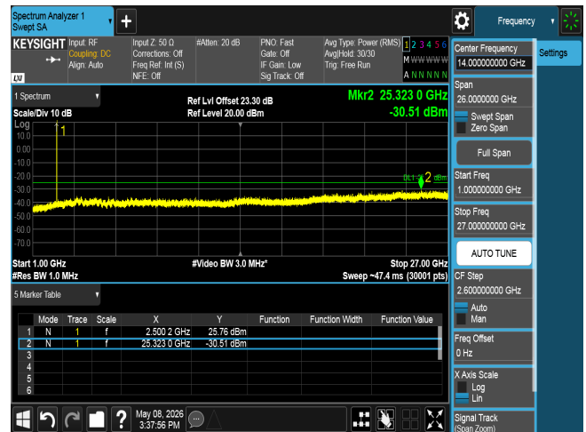
CSE n7 10M CH501000 BPSK(1,1)
