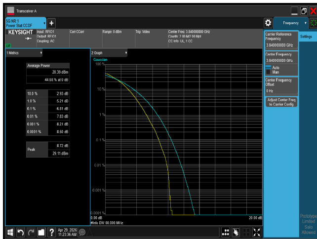
PTAR n77 80M CH656000 64QAM
