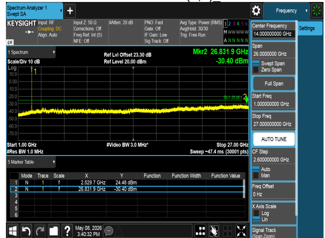
CSE n7 10M CH507000 BPSK(1,1)
