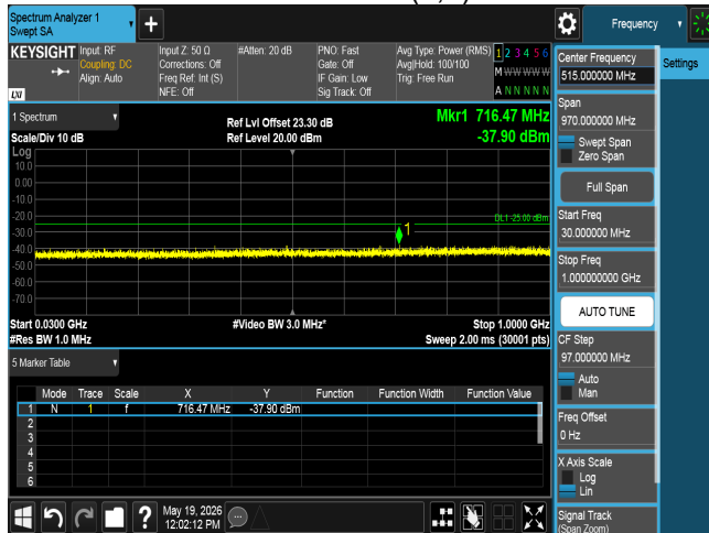
CSE n7 20M CH512000 BPSK(1,1)
