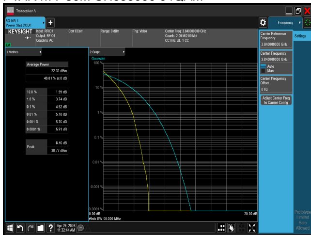
PTAR n77 90M CH656000 BPSK
