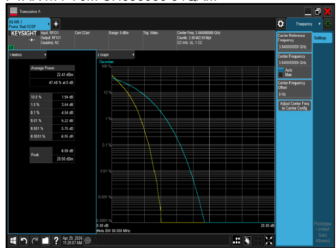
PTAR n77 80M CH656000 BPSK
