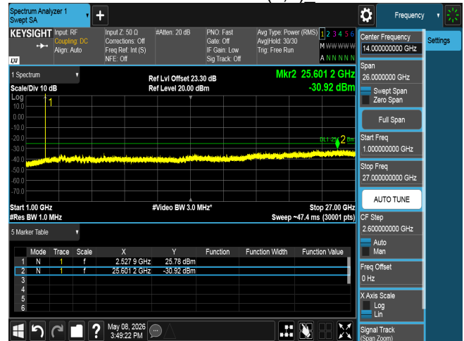
CSE n7 15M CH507000 BPSK(1,1)
