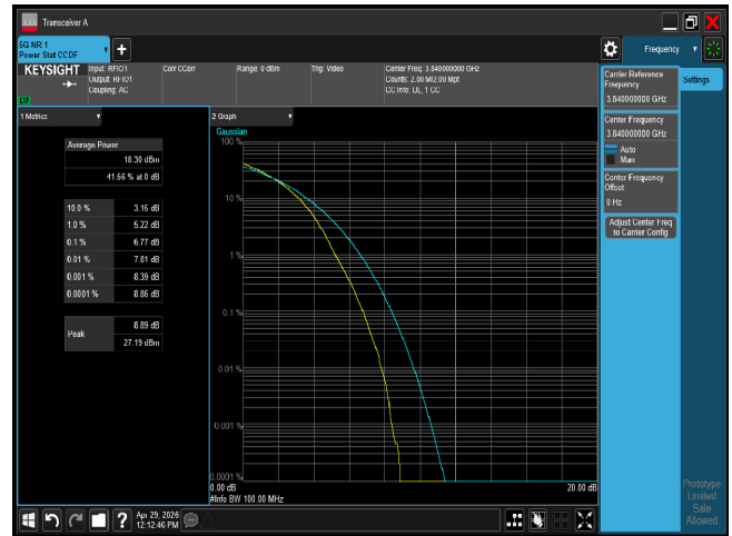
PTAR n77 100M CH656000 256QAM
