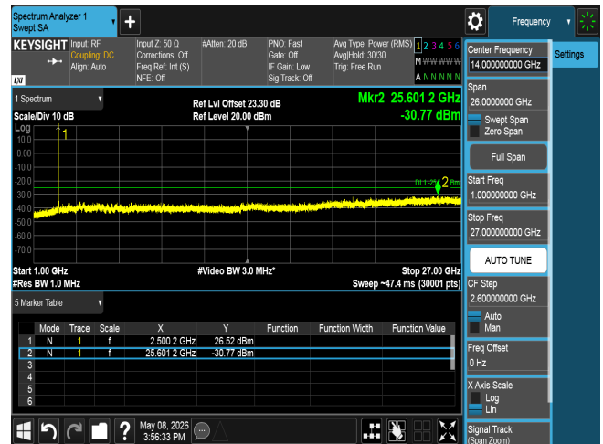
CSE n7 20M CH502000 BPSK(1,1)
