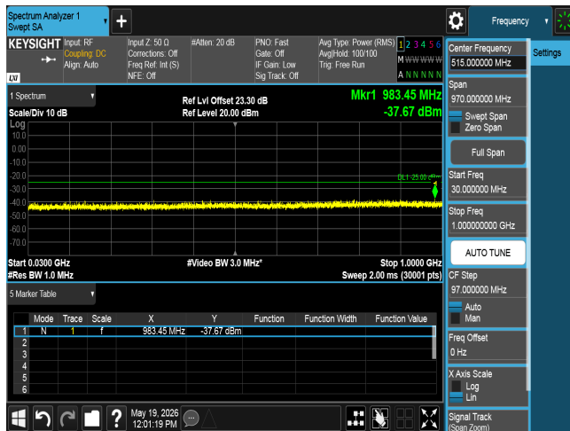
CSE n7 20M CH502000 BPSK(1,1)
