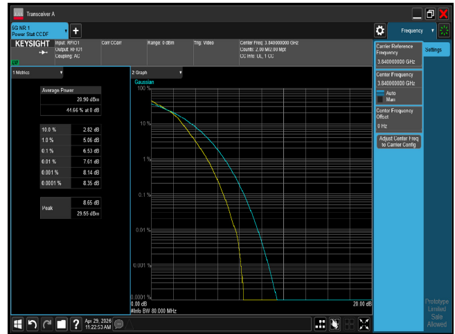
PTAR n77 80M CH656000 16QAM
