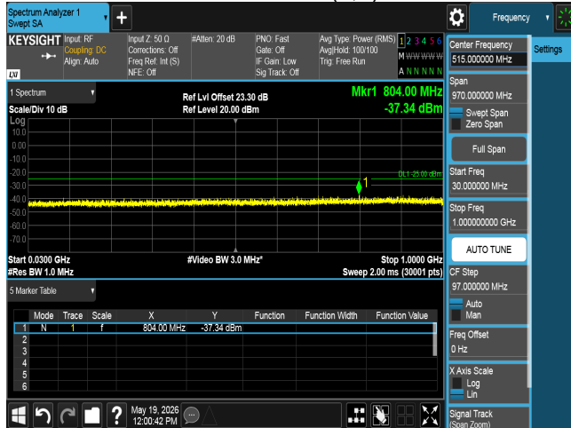
CSE n7 15M CH512500 BPSK(1,1)
