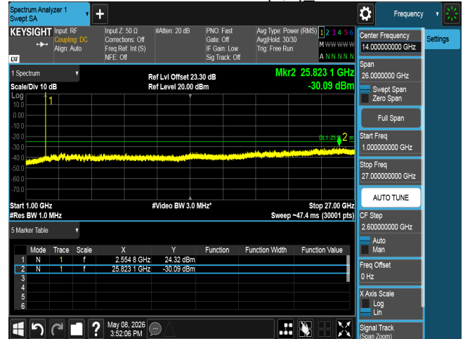
CSE n7 15M CH512500 BPSK(1,1)_
