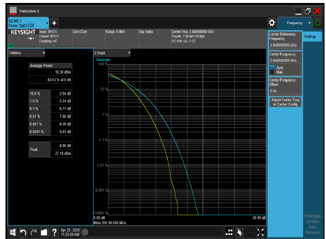
PTAR n77 80M CH656000 256QAM
