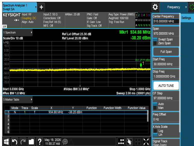
CSE n7 10M CH501000 BPSK(1,1)
