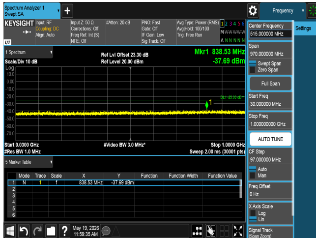
CSE n7 15M CH501500 BPSK(1,1)
