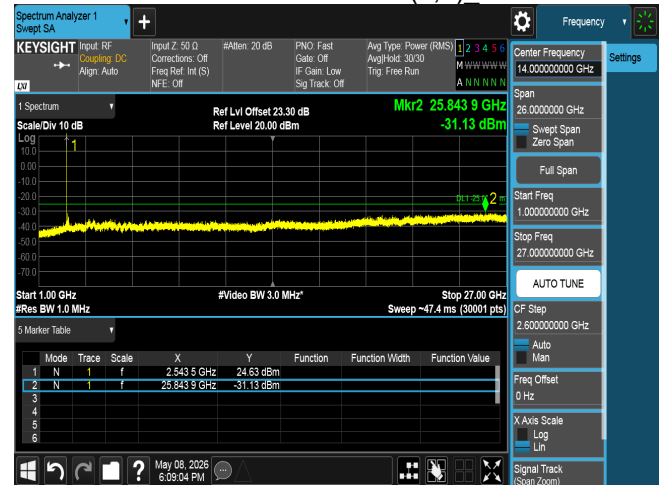
CSE n41 100M CH518598 BPSK(1,1)
