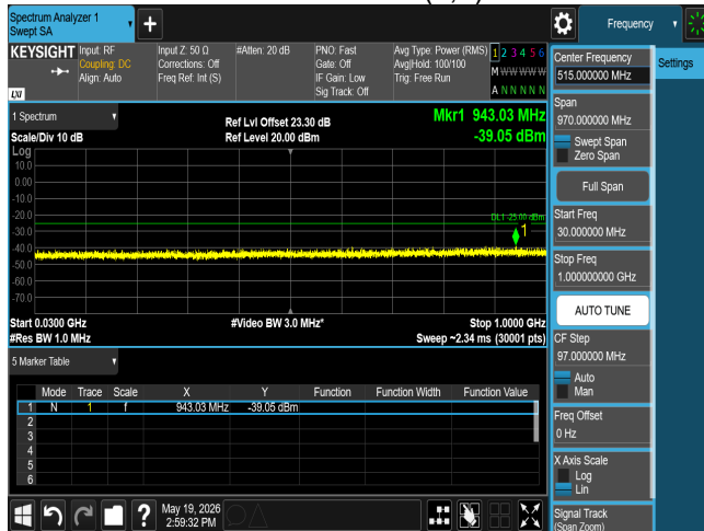
CSE n41 80M CH518598 BPSK(1,1)
