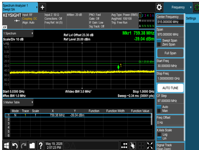
CSE n41 80M CH507204 BPSK(1,1)
