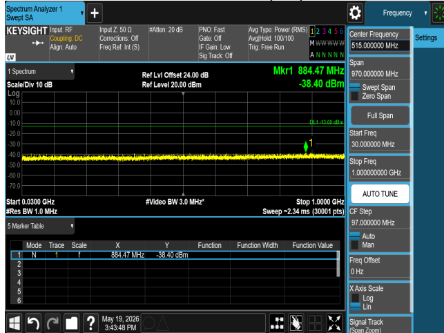
CSE n77 50M CH633334 BPSK(1,1)
