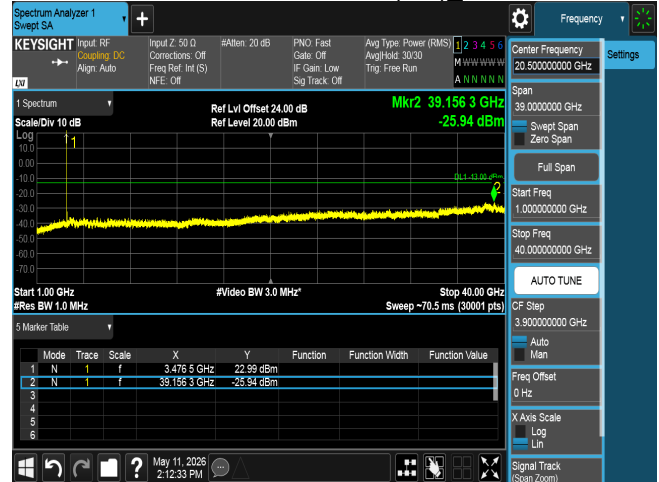
CSE n77 50M CH633334 BPSK(1,1)
