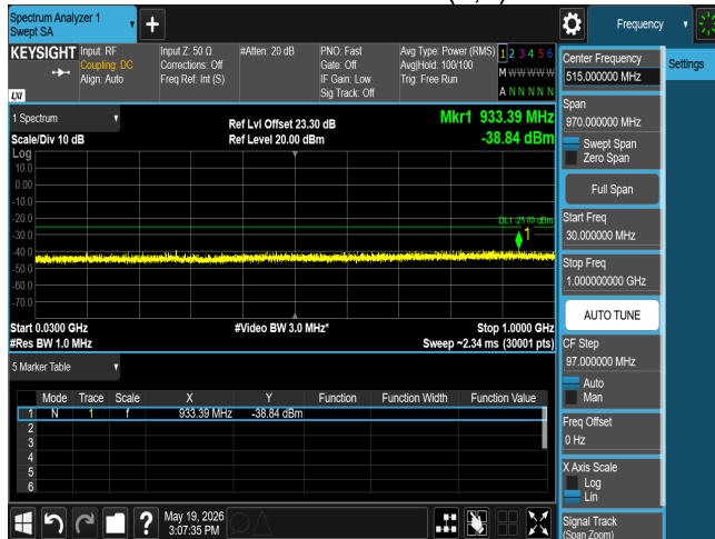
CSE n41 100M CH518598 BPSK(1,1)
