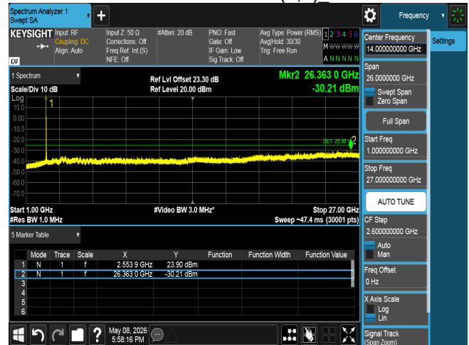
CSE n41 80M CH518598 BPSK(1,1)
