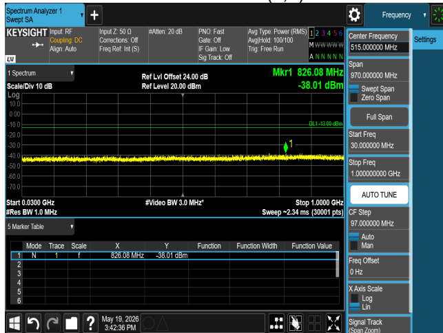
CSE n77 40M CH635332 BPSK(1,1)
