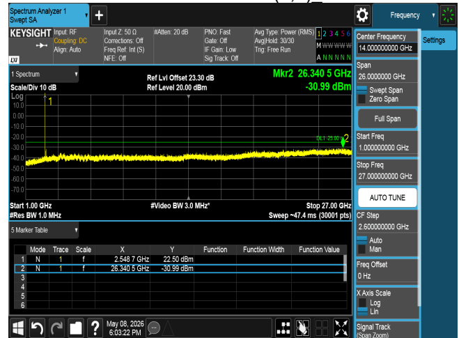
CSE n41 90M CH518598 BPSK(1,1)
