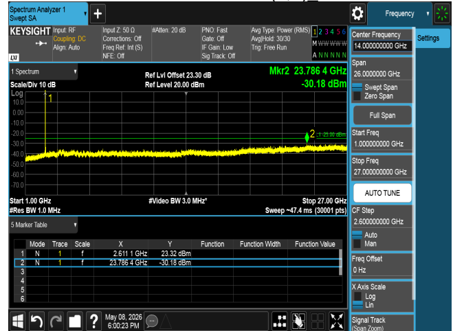
CSE n41 80M CH529998 BPSK(1,1)_
