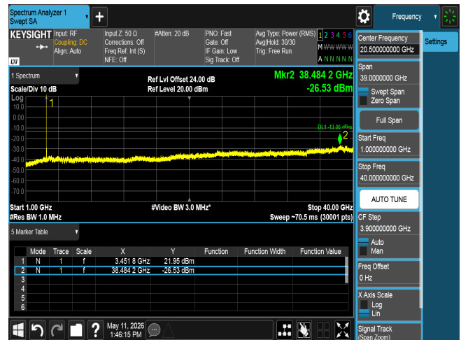
CSE n77 50M CH631668 BPSK(1,1)
