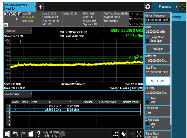
CSE n41 80M CH507204 BPSK(1,1)
