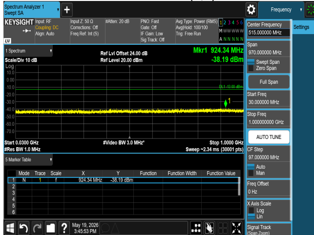
CSE n77 50M CH635000 BPSK(1,1)
