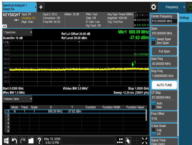
CSE n77 50M CH631668 BPSK(1,1)
