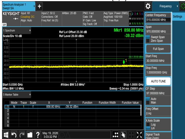
CSE n41 90M CH518598 BPSK(1,1)
